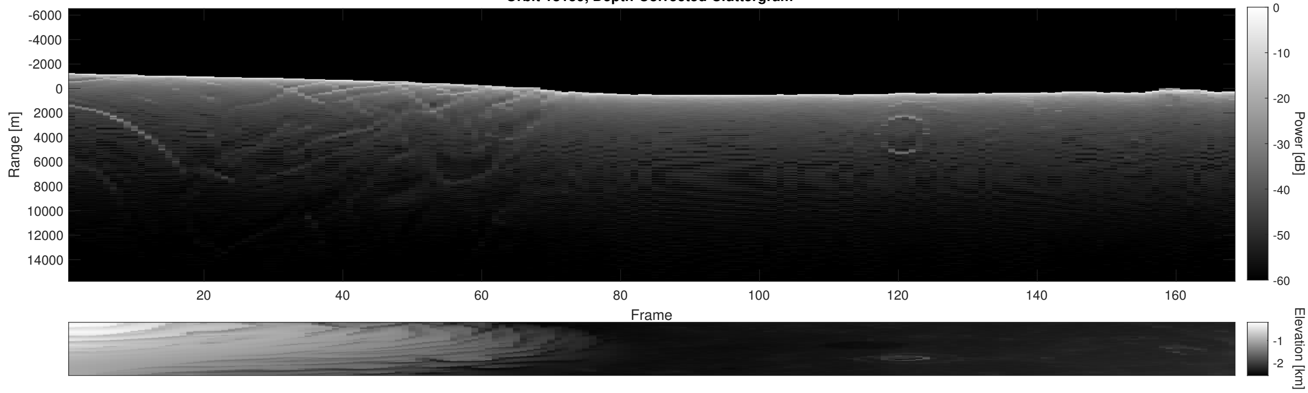
Orbit 18159, Depth-Corrected Cluttergram
