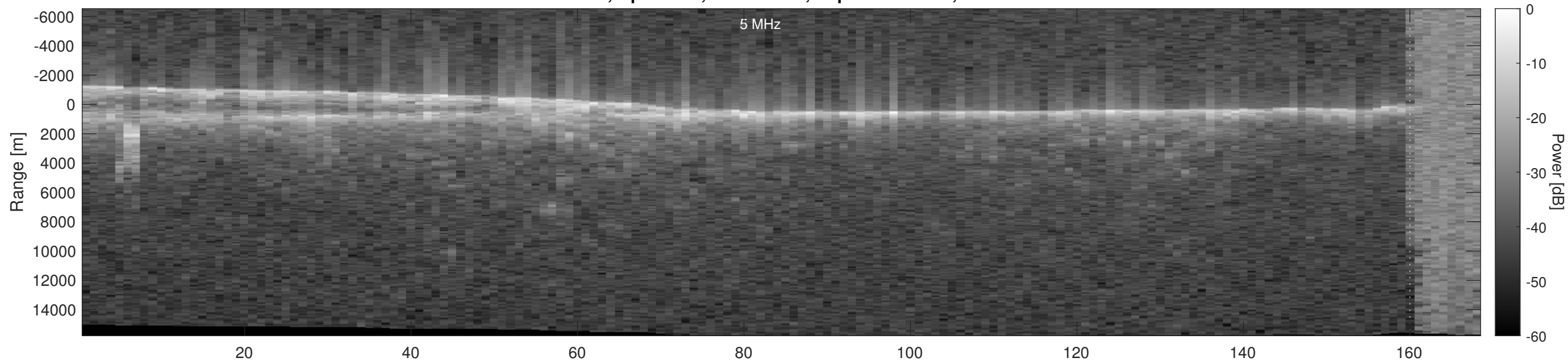
Orbit 18159, Optimized, No Window, Depth-Corrected, Channel 2
