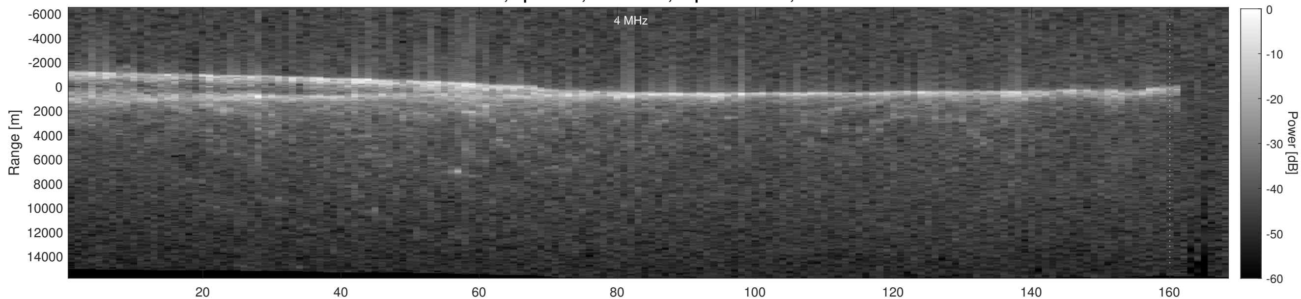
Orbit 18159, Depth-Corrected Cluttergram
