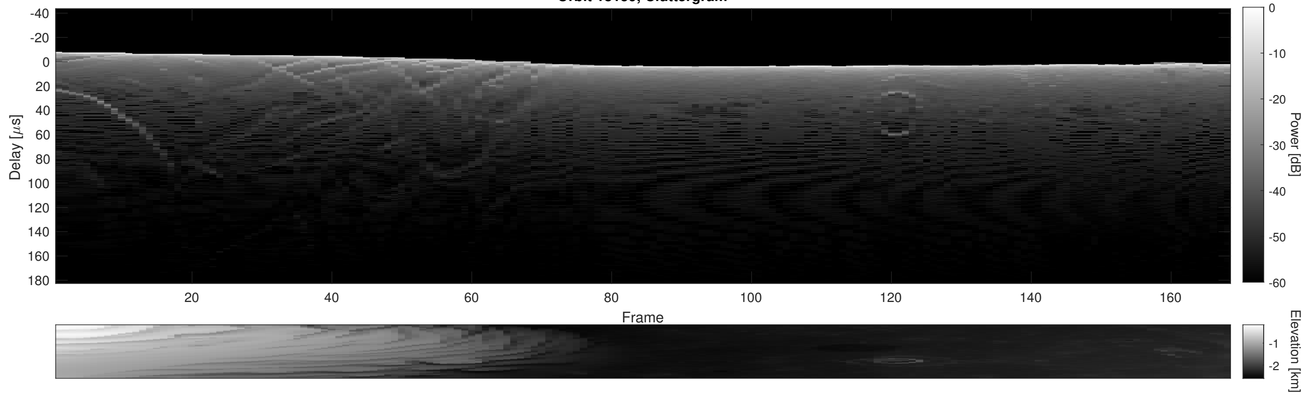
Orbit 18159, Cluttergram
