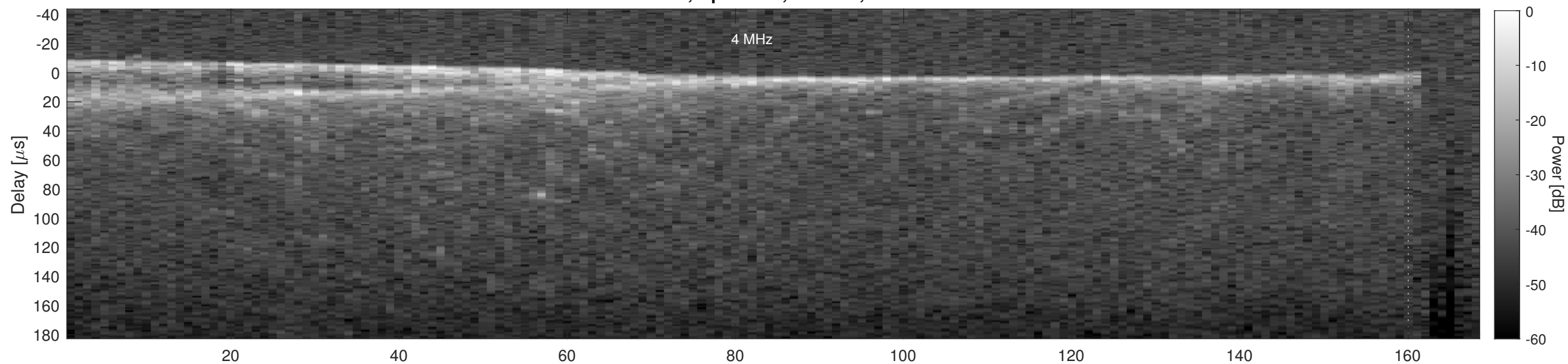
Orbit 18159, Cluttergram
