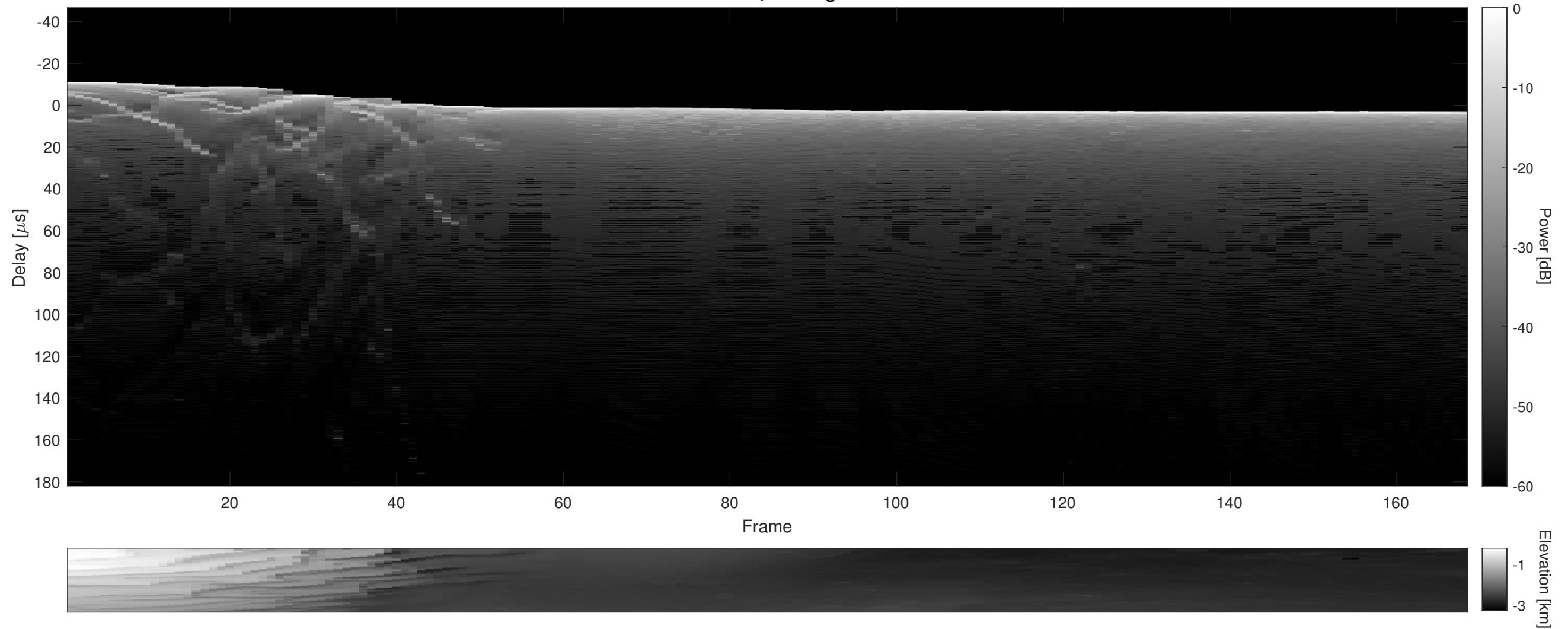
Orbit 18162, Cluttergram
