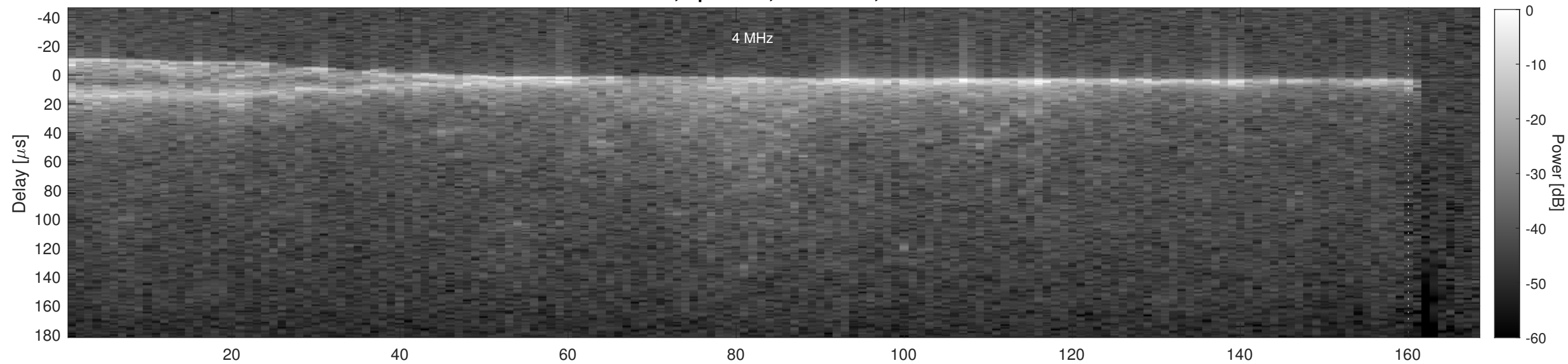
Orbit 18162, Cluttergram
