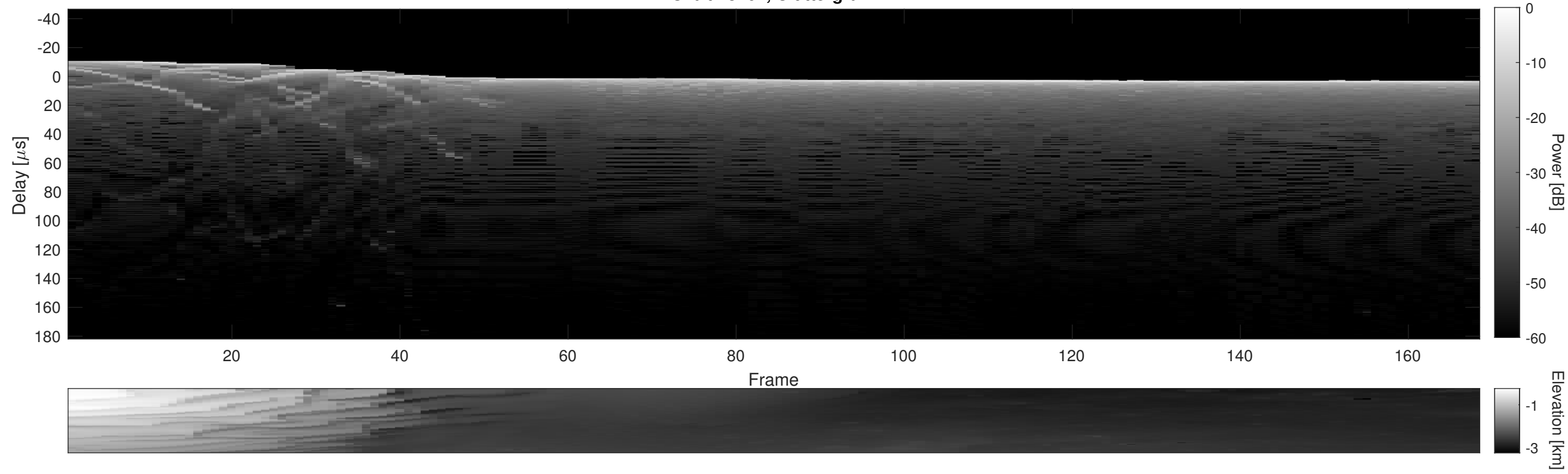
Orbit 18162, Cluttergram
