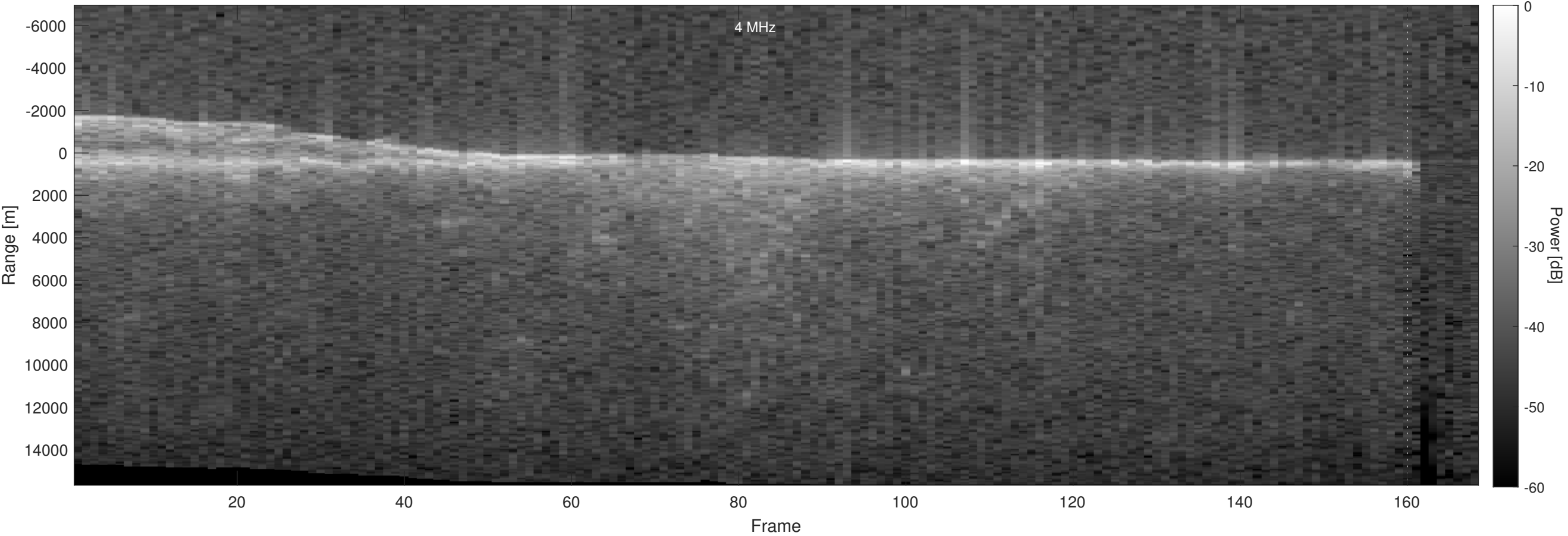
Orbit 18162, Optimized, No Window, Depth-Corrected, Channel 2
