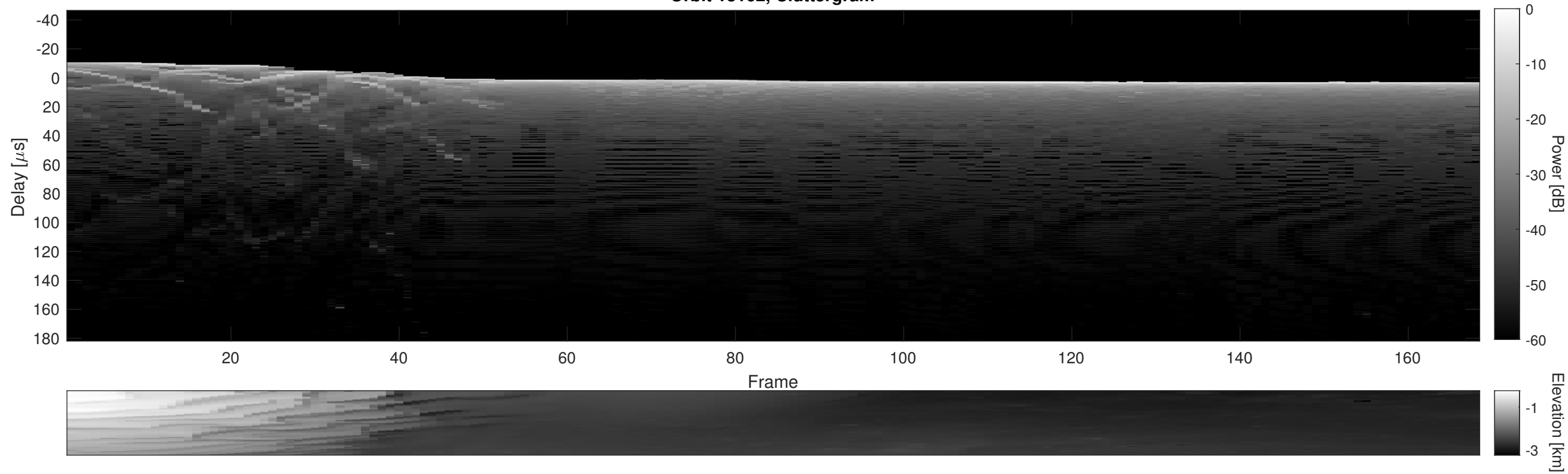
Orbit 18162, Cluttergram
