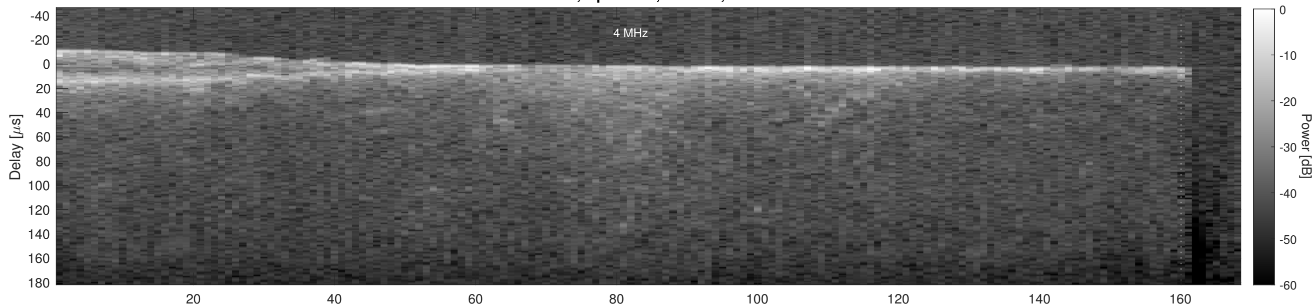
Orbit 18162, Cluttergram
