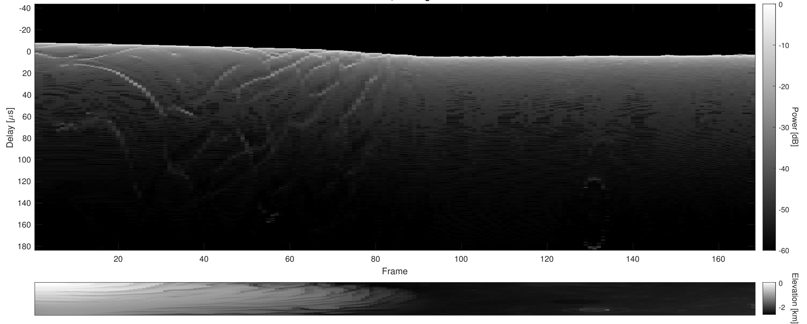
Orbit 18166, Cluttergram
