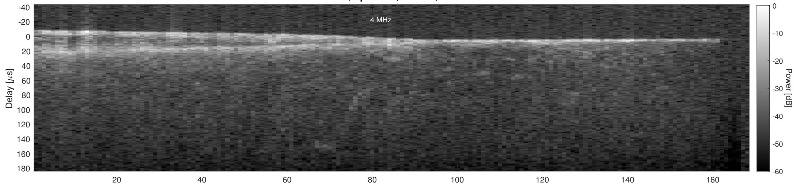
Orbit 18166, Cluttergram
