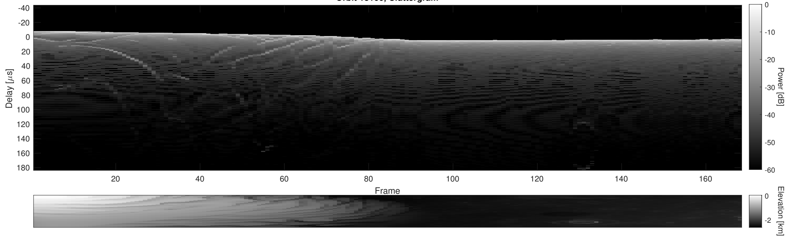
Orbit 18166, Cluttergram
