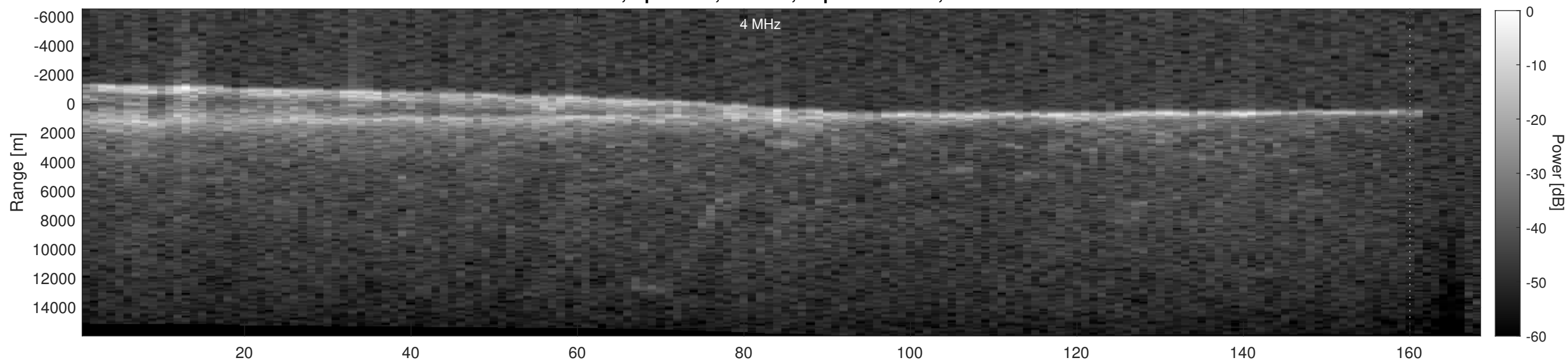
Orbit 18166, Depth-Corrected Cluttergram
