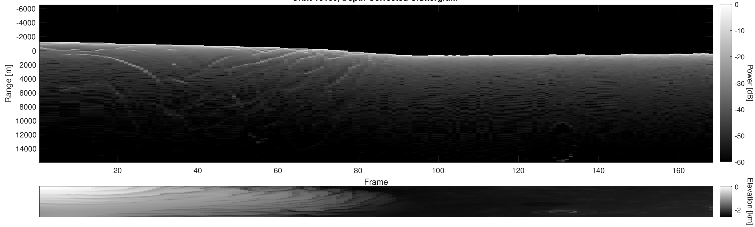
Orbit 18166, Depth-Corrected Cluttergram
