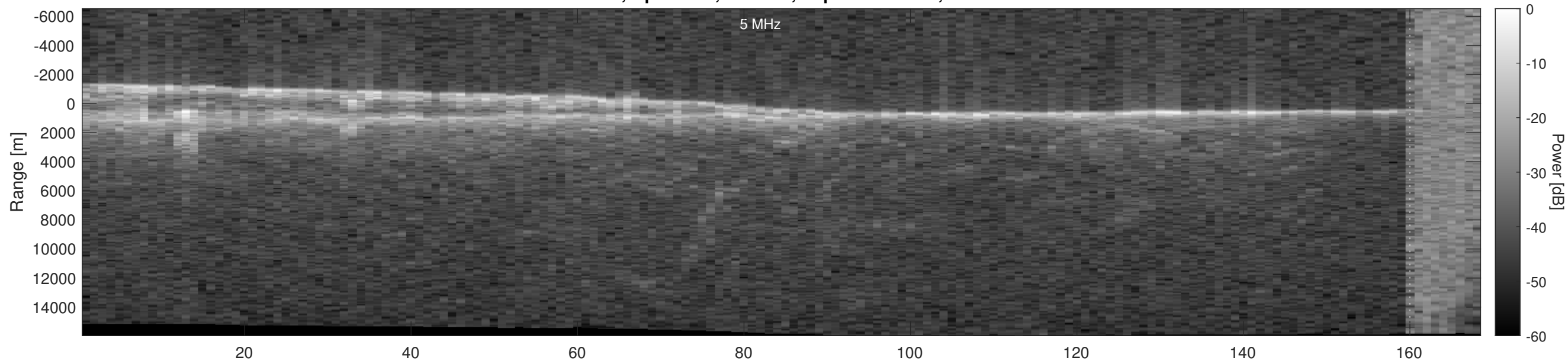
Orbit 18166, Optimized, Window, Depth-Corrected, Channel 2
