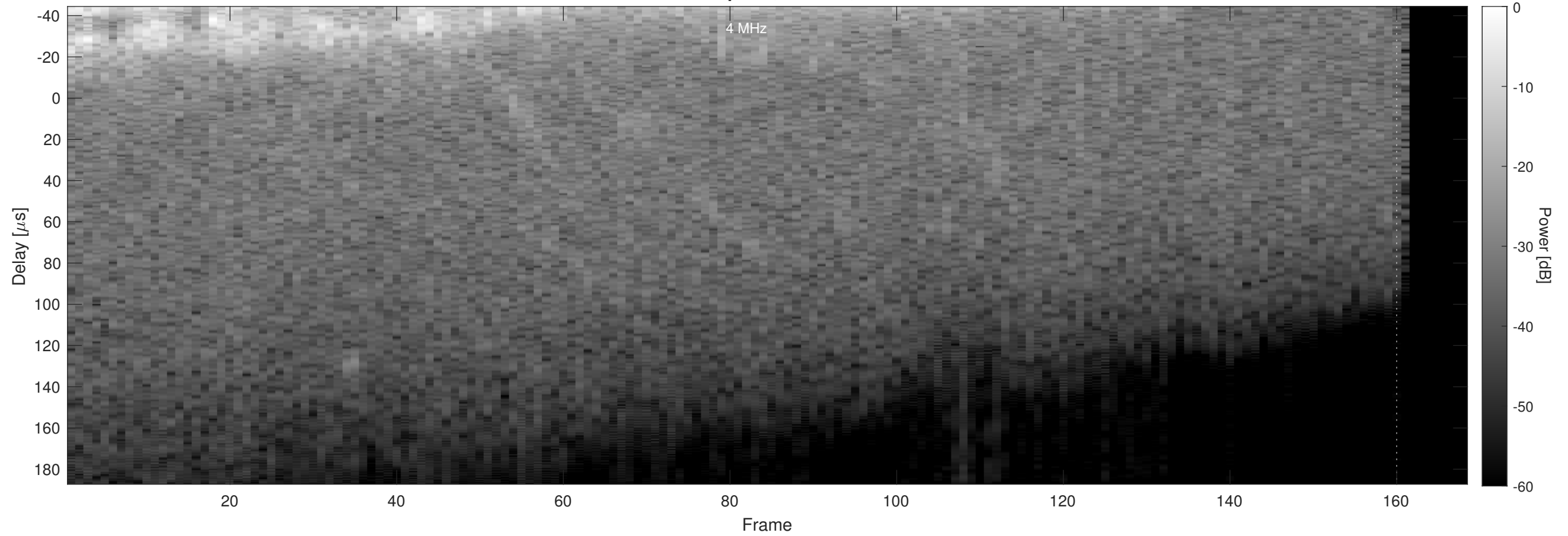
Orbit 18174, Chapman, Window, Channel 2
