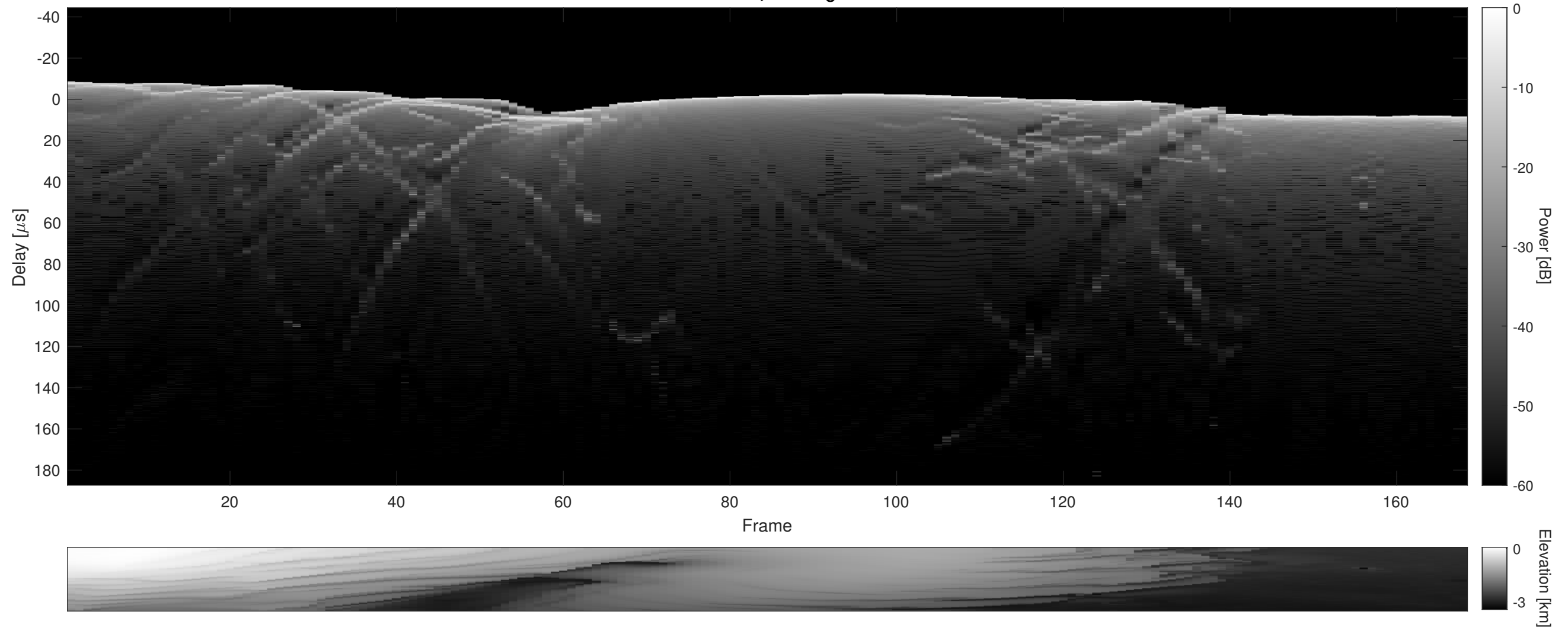
Orbit 18174, Cluttergram
