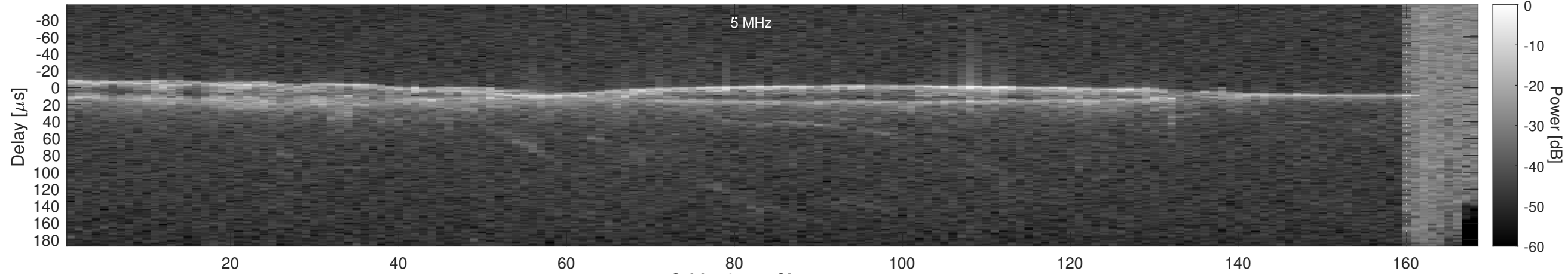
Orbit 18174, Cluttergram
