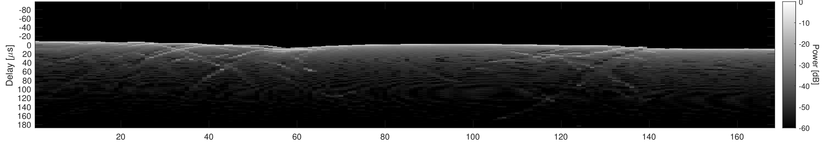
Orbit 18174, Cluttergram
