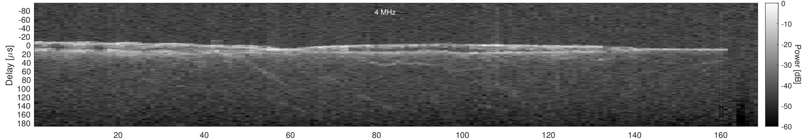
Orbit 18174, Cluttergram
