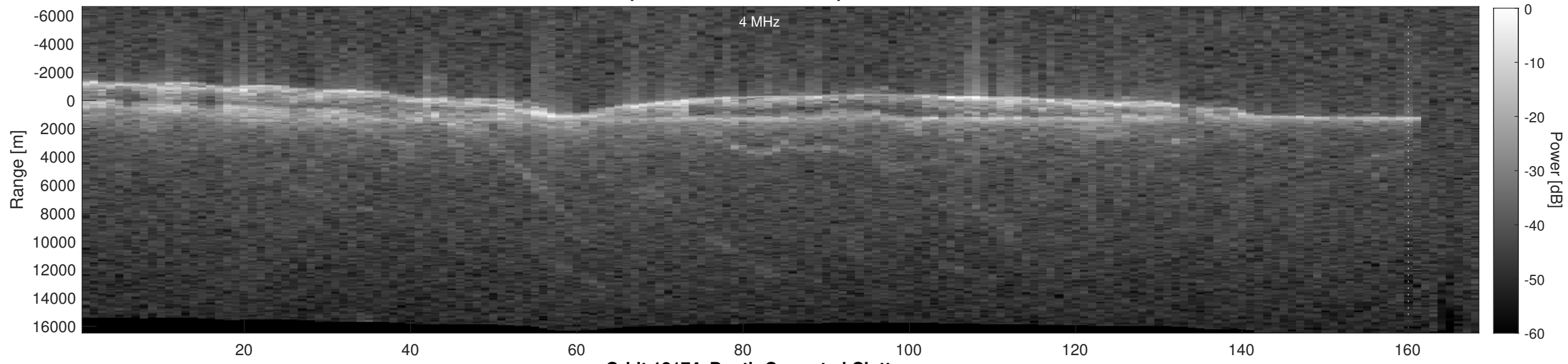
Orbit 18174, Depth-Corrected Cluttergram
