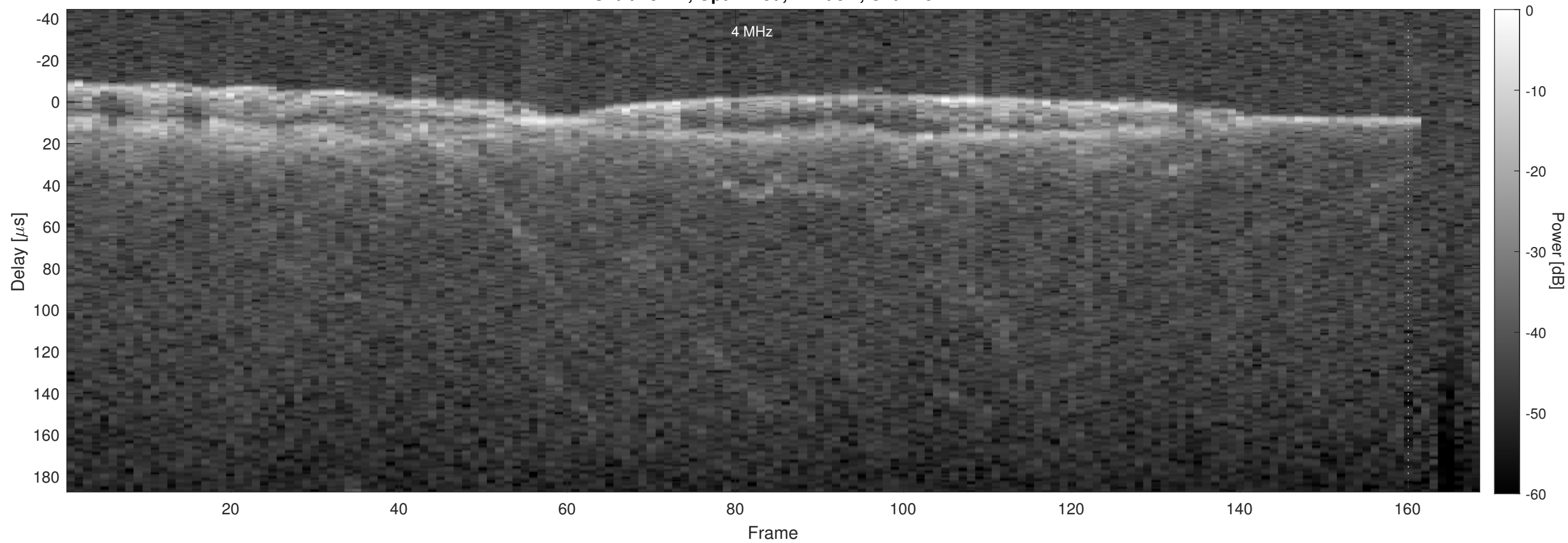
Orbit 18174, Optimized, Window, Channel 2
