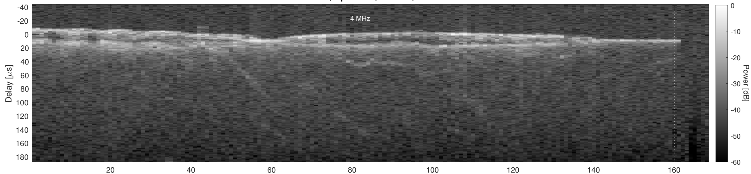
Orbit 18174, Cluttergram
