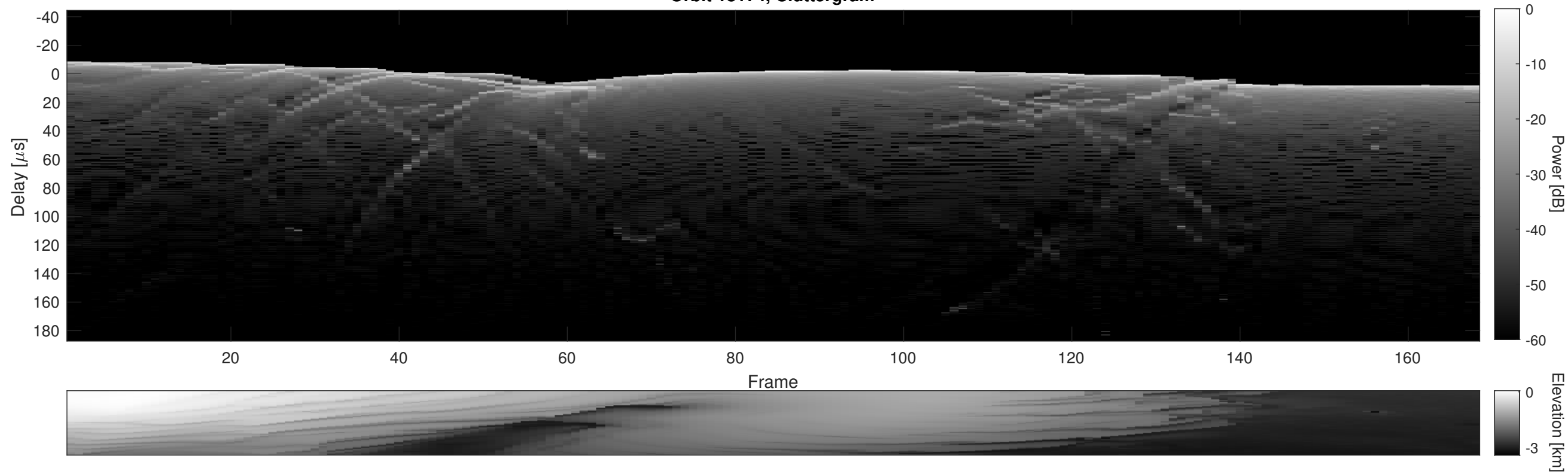
Orbit 18174, Cluttergram
