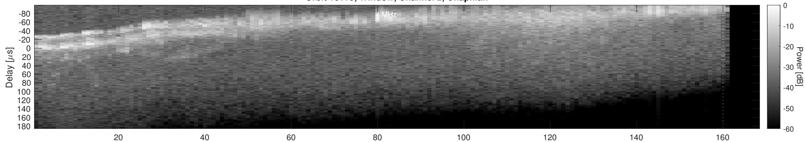
Orbit 18179, Window, Channel 2, Optimized
