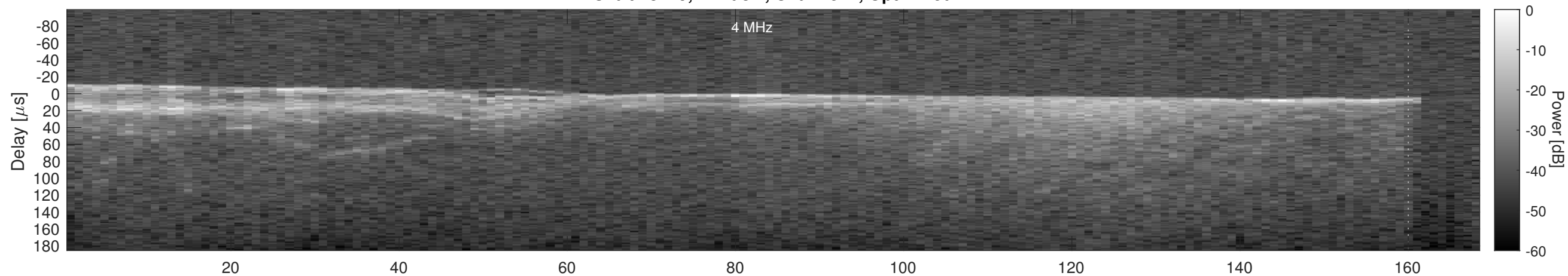
Orbit 18179, Cluttergram
