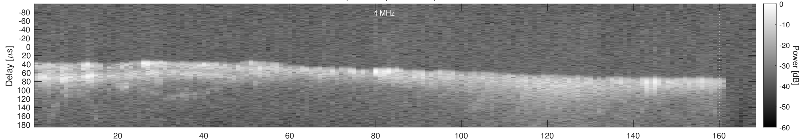
Orbit 18179, Window, Channel 2, Chapman
