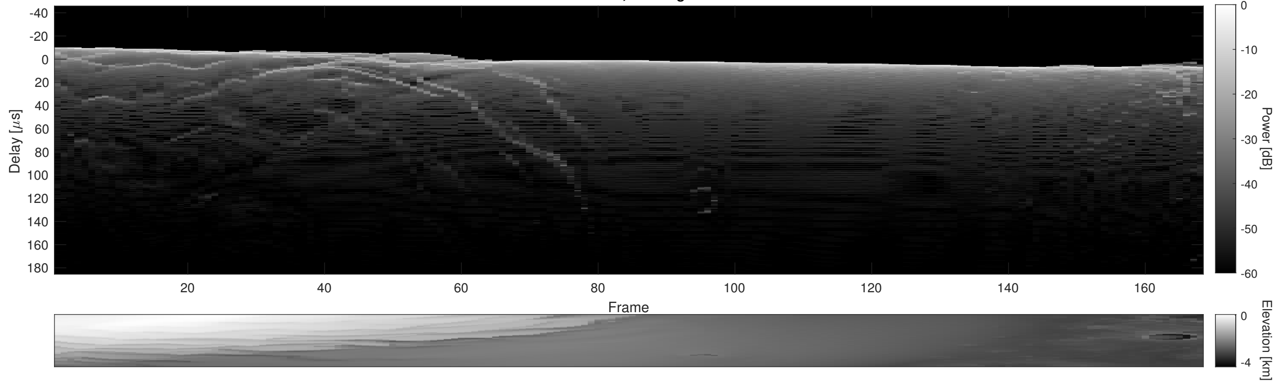
Orbit 18179, Cluttergram
