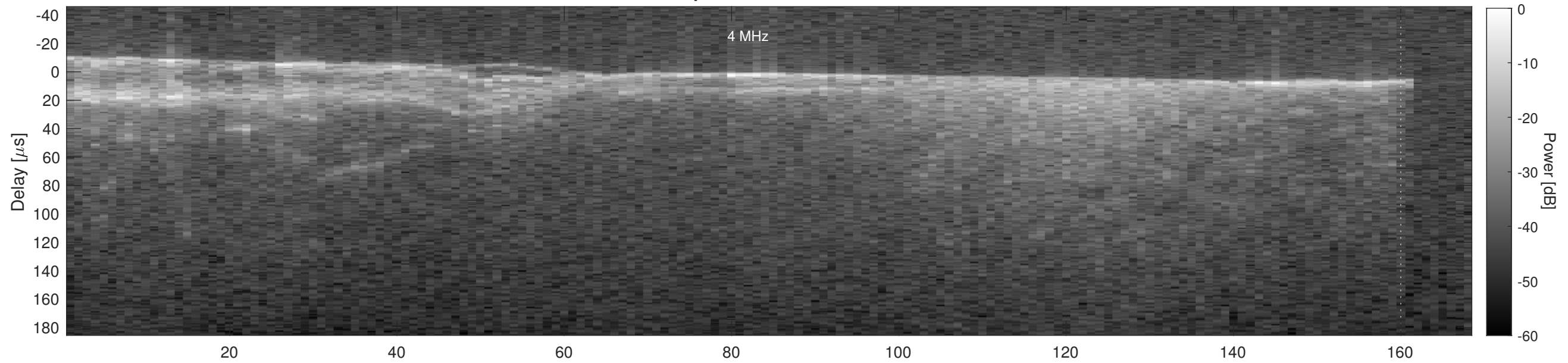
Orbit 18179, Cluttergram
