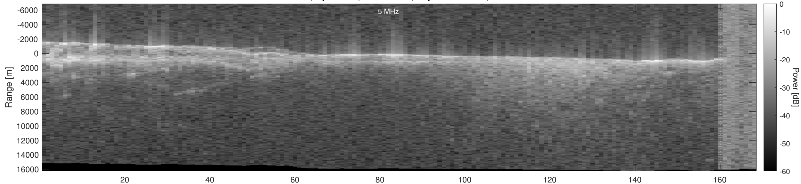
Orbit 18179, Optimized, No Window, Depth-Corrected, Channel 2
