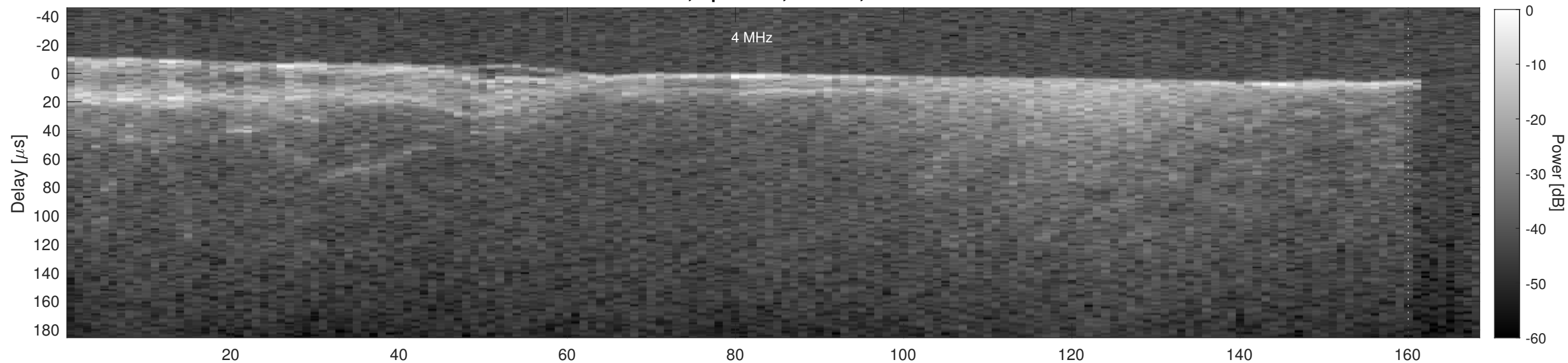
Orbit 18179, Cluttergram
