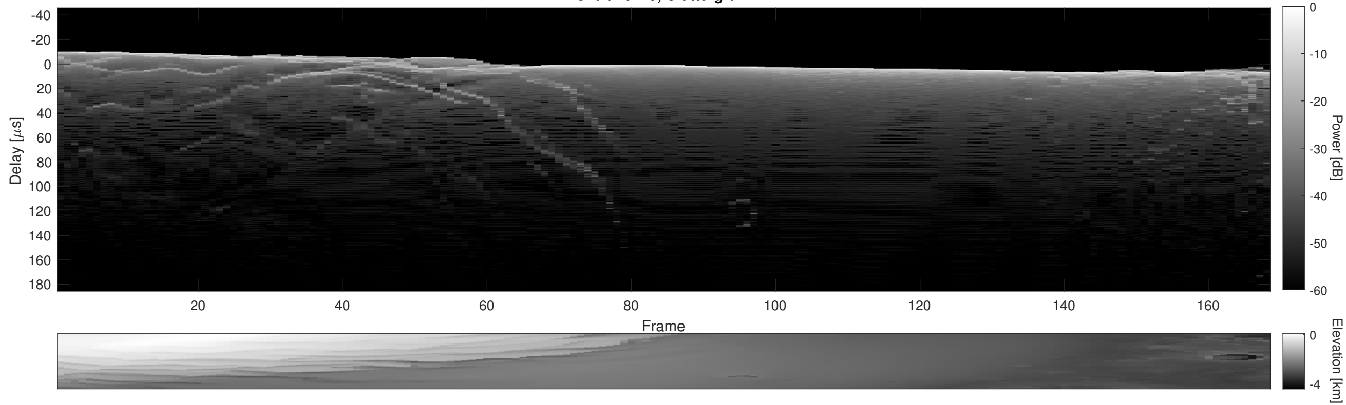
Orbit 18179, Cluttergram
