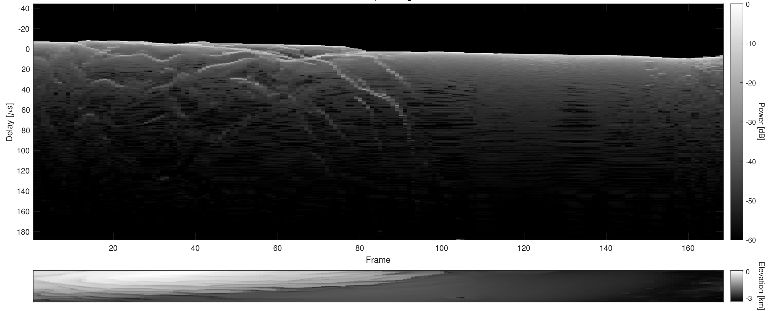
Orbit 18186, Cluttergram
