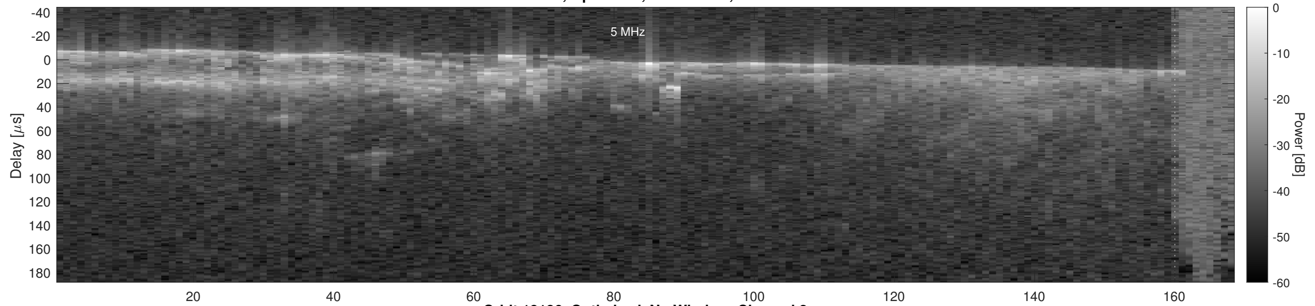
Orbit 18186, Optimized, No Window, Channel 2
