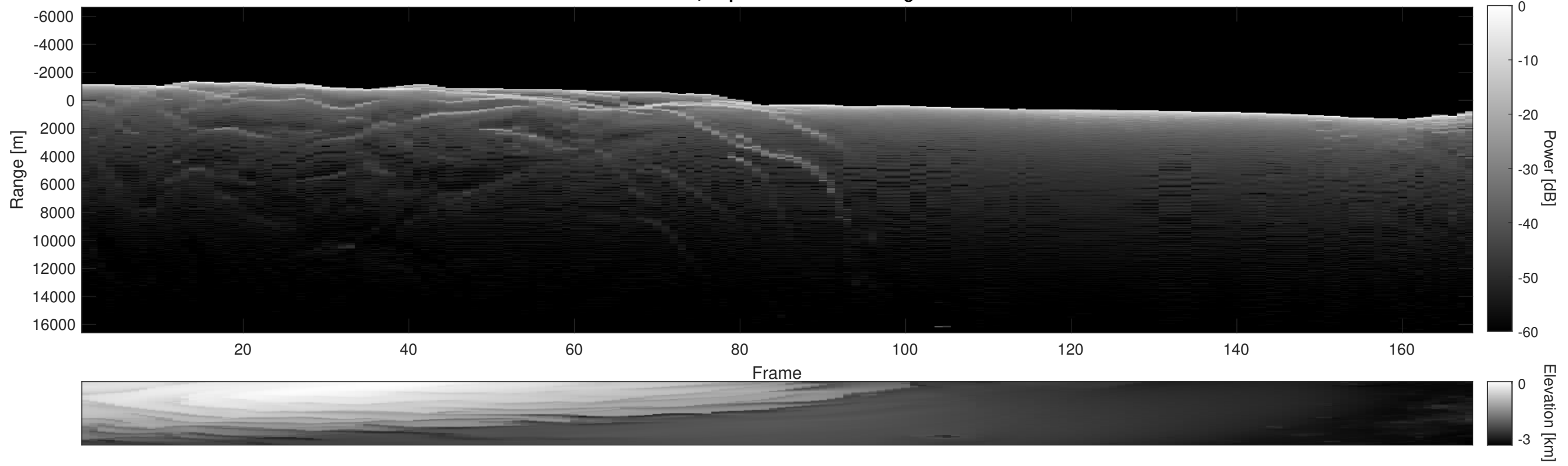
Orbit 18186, Depth-Corrected Cluttergram
