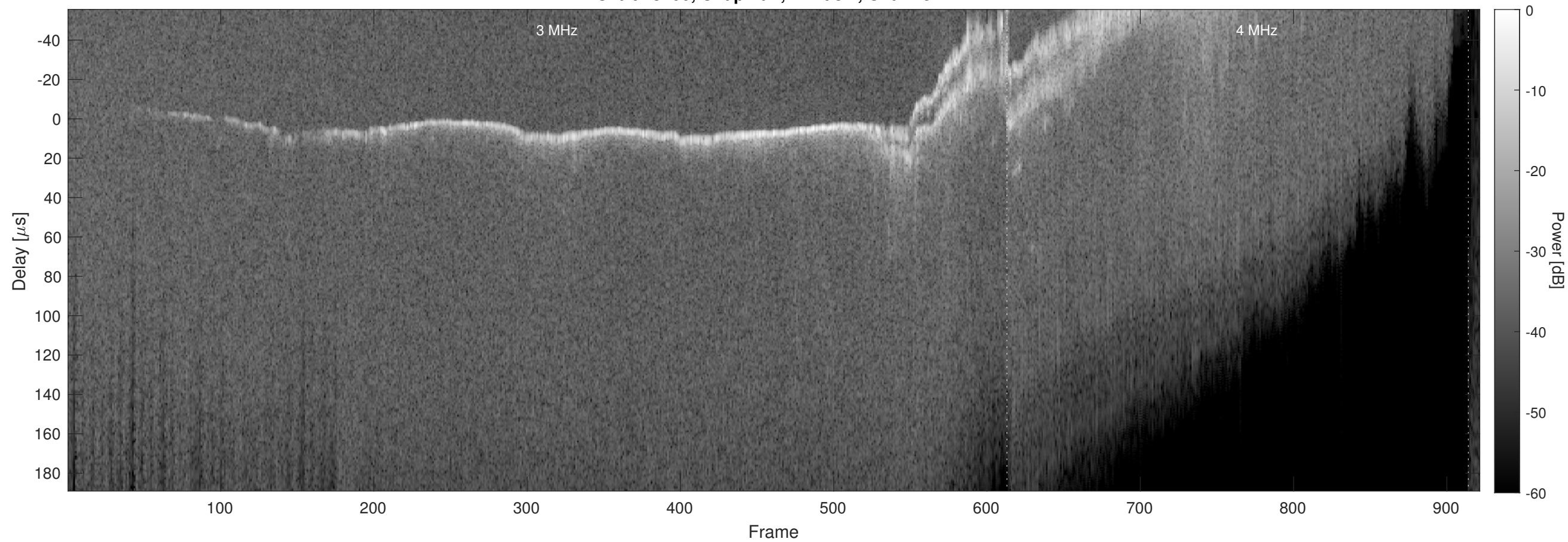
Orbit 18200, Chapman, Window, Channel 2
