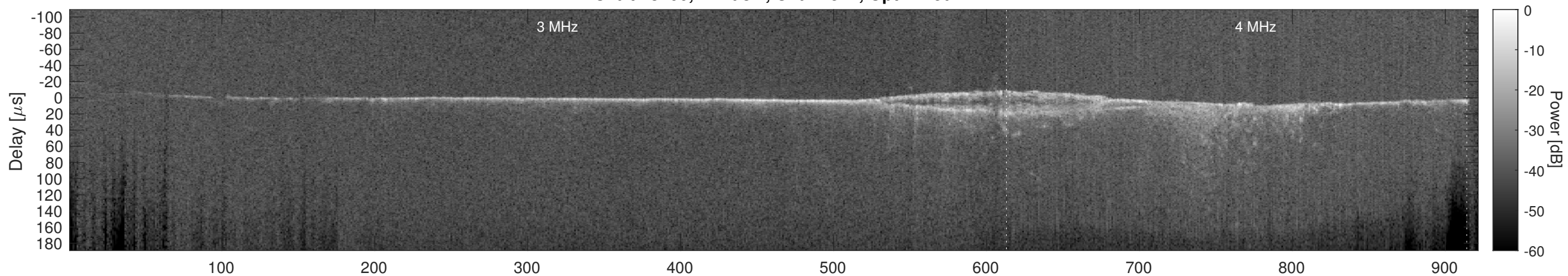
Orbit 18200, Cluttergram
