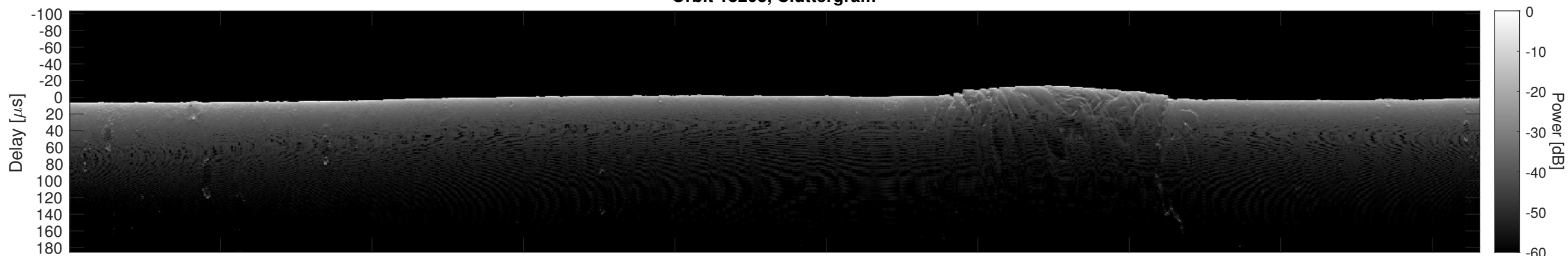
Orbit 18203, Cluttergram
