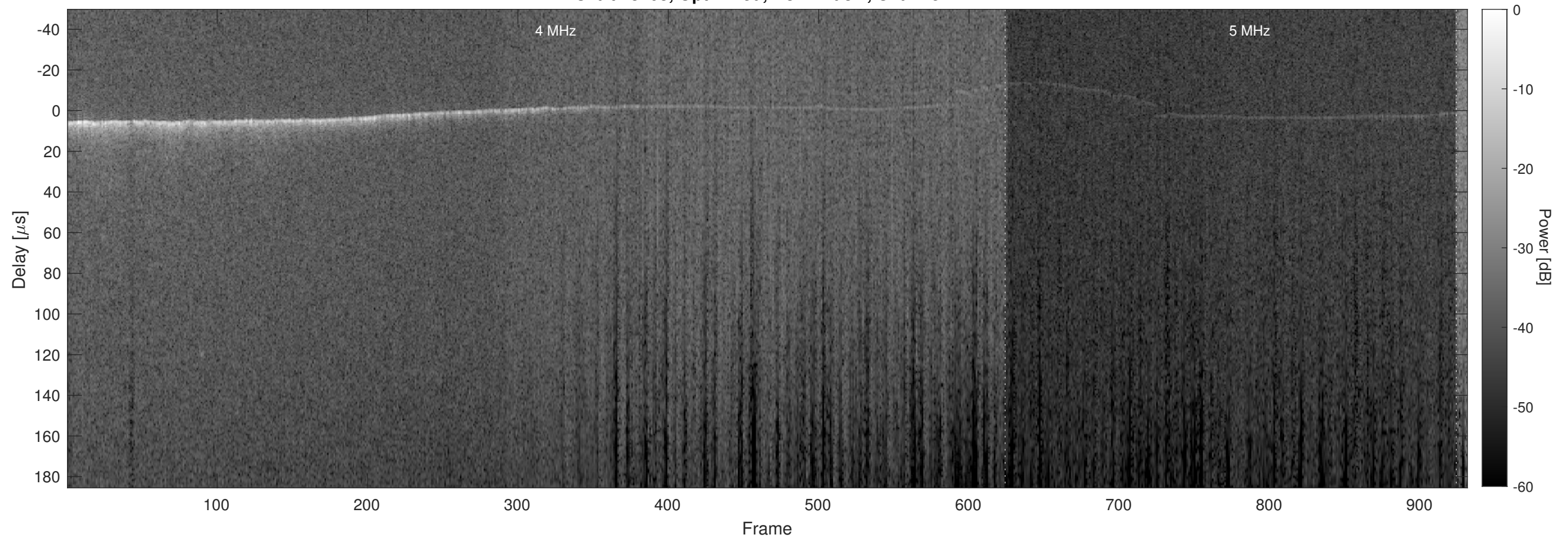
Orbit 18203, Optimized, No Window, Channel 2
