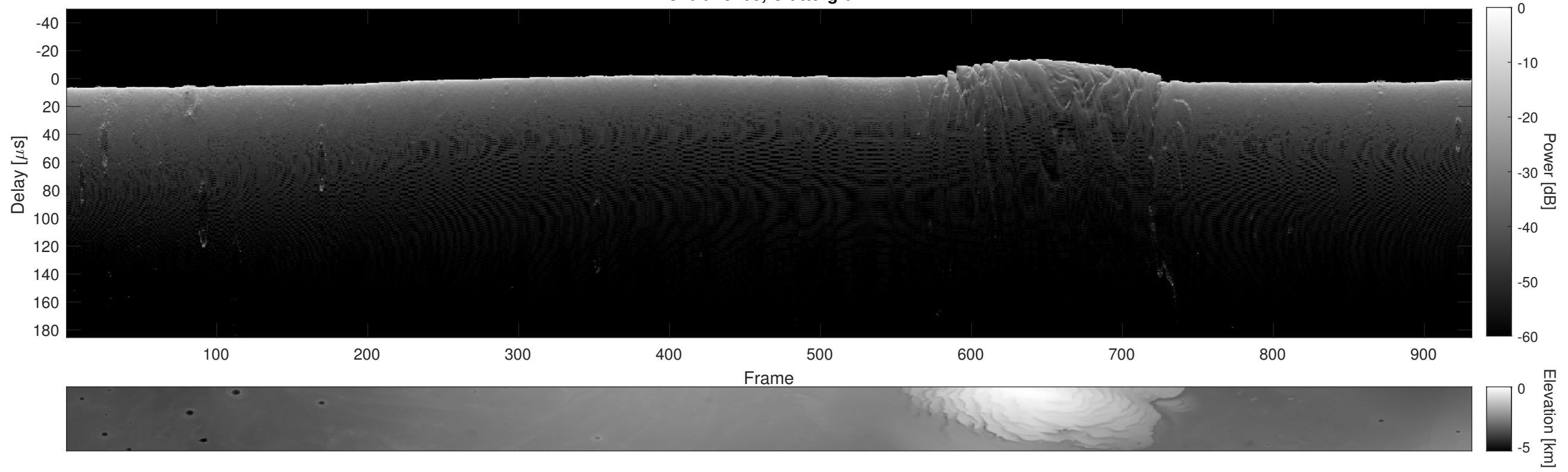
Orbit 18203, Cluttergram
