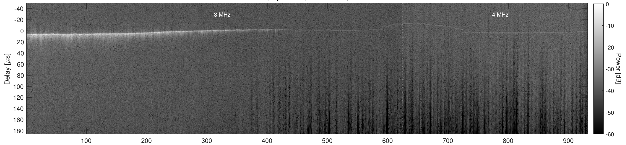
Orbit 18203, Cluttergram
