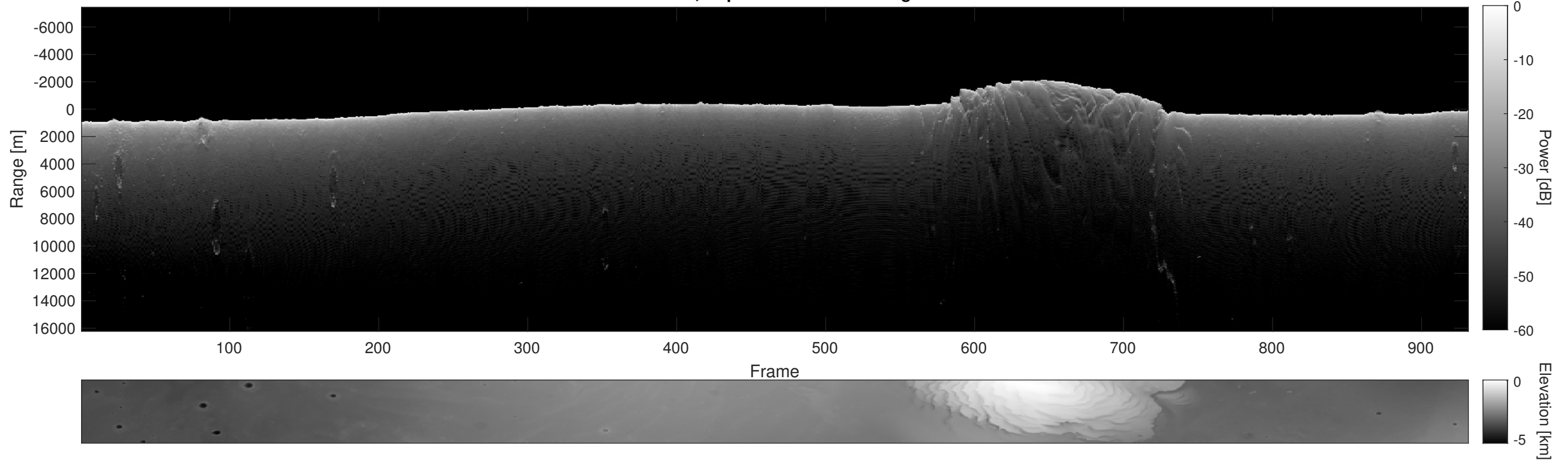
Orbit 18203, Depth-Corrected Cluttergram
