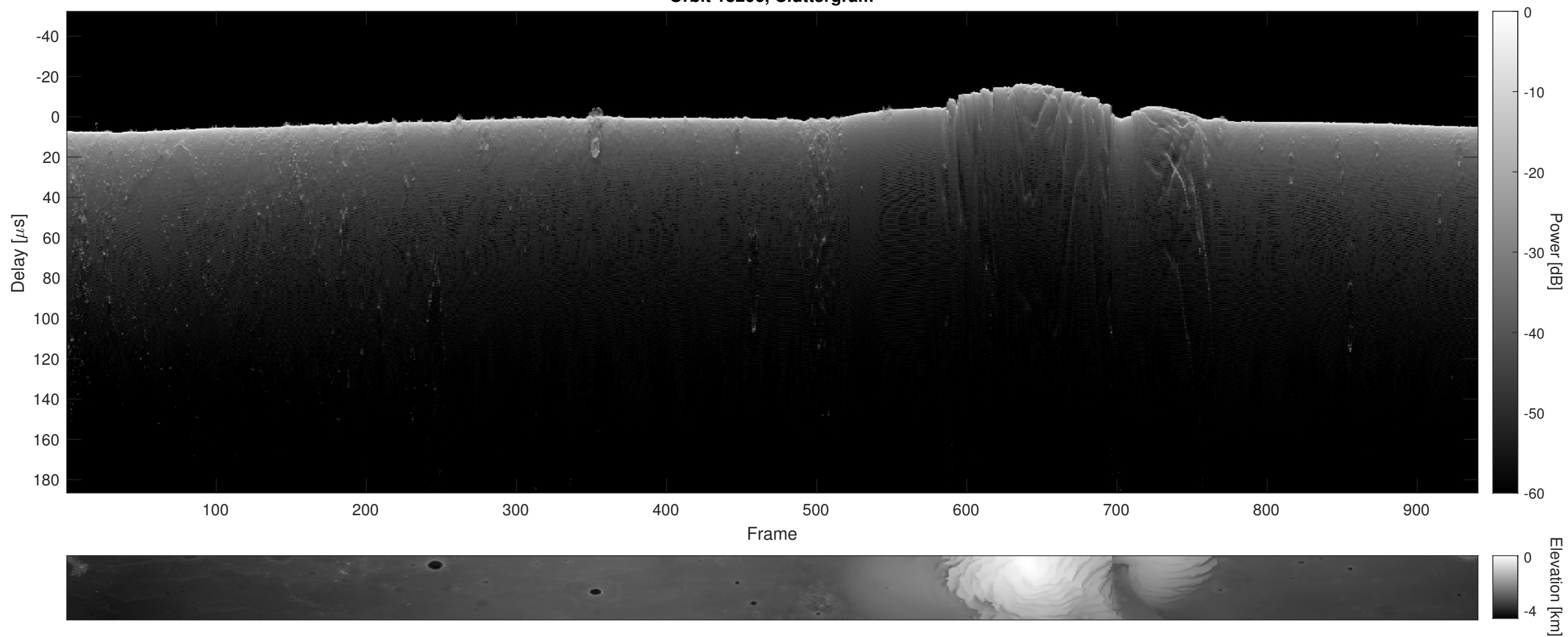
Orbit 18206, Cluttergram
