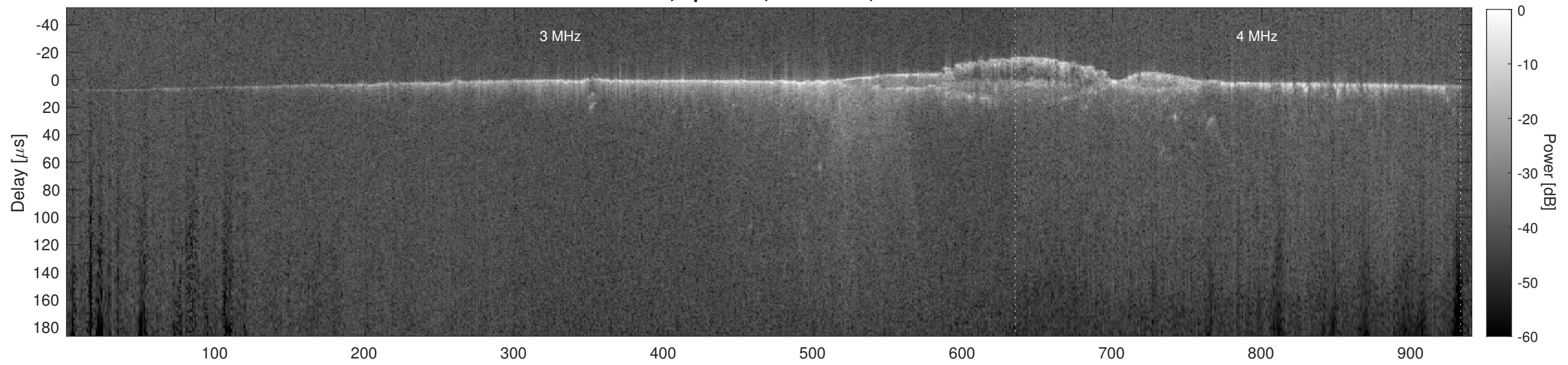
Orbit 18206, Cluttergram
