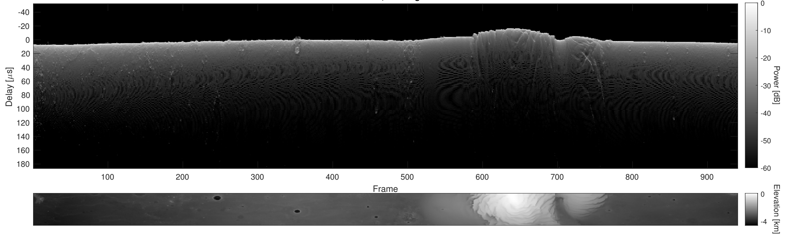
Orbit 18206, Cluttergram
