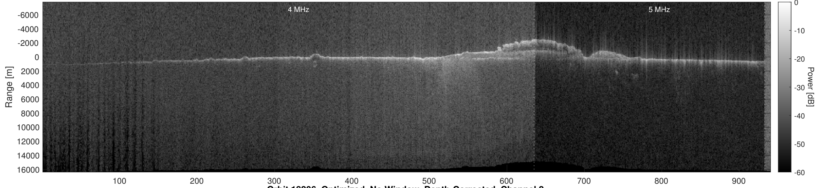
Orbit 18206, Optimized, No Window, Depth-Corrected, Channel 2
