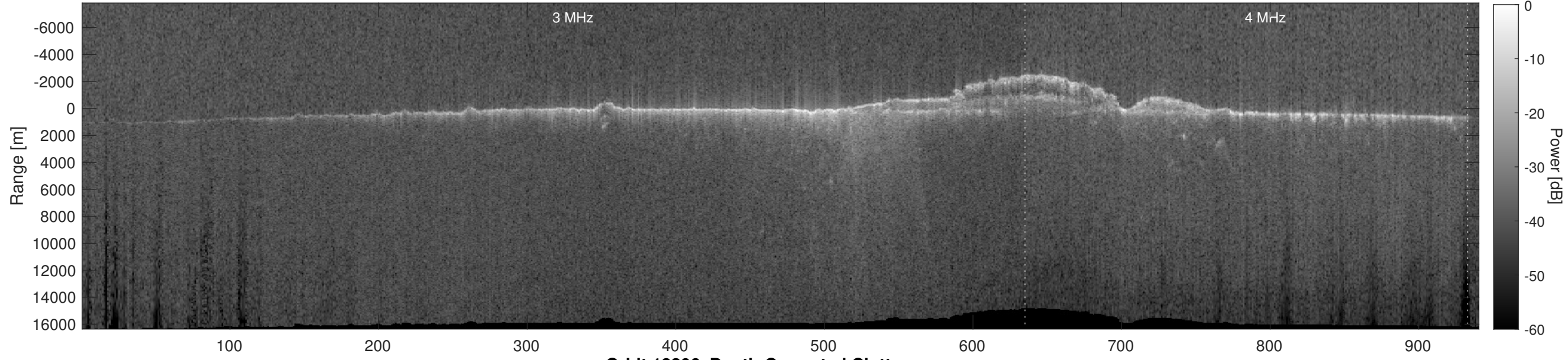
Orbit 18206, Depth-Corrected Cluttergram
