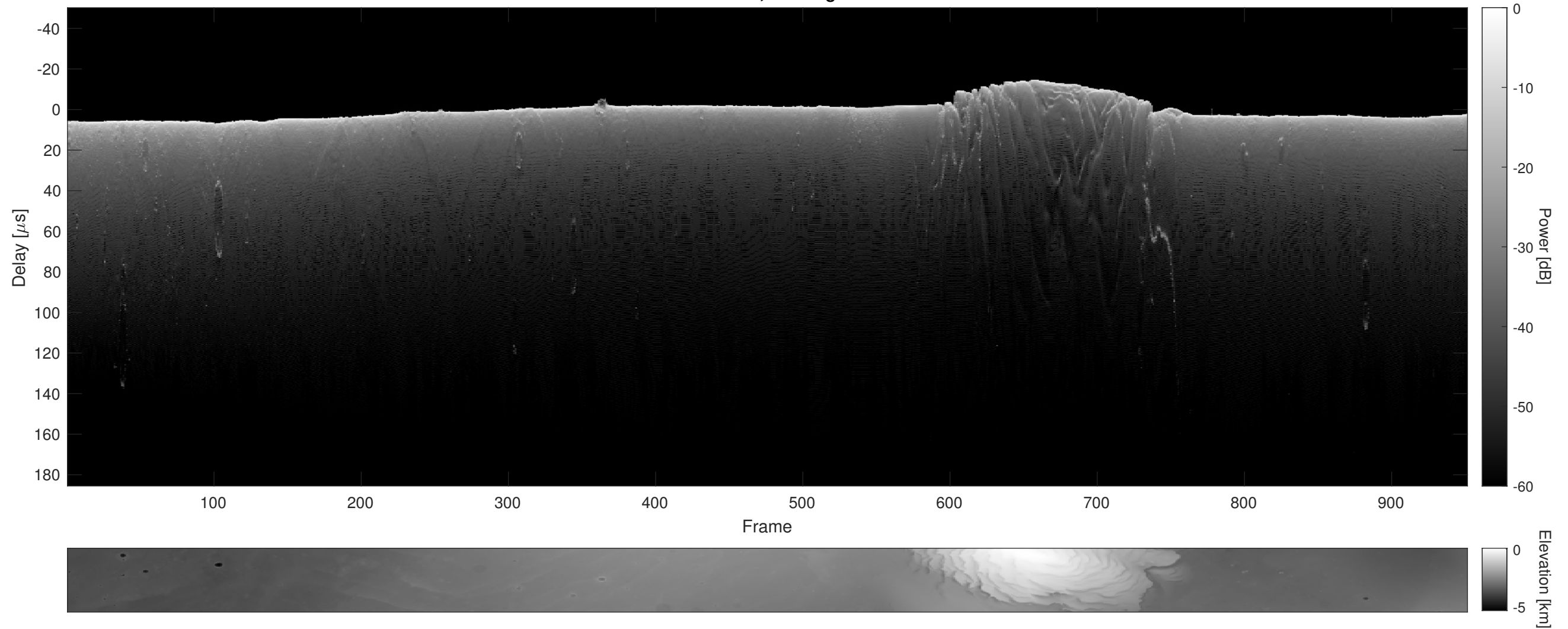
Orbit 18210, Cluttergram
