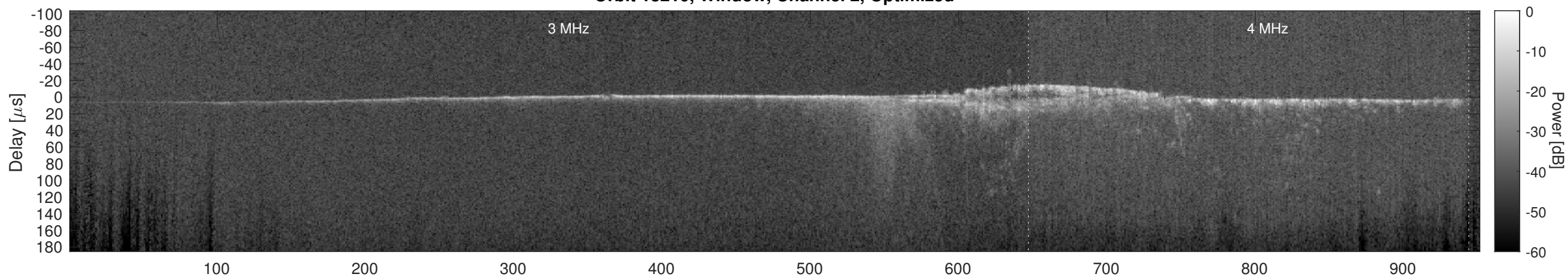
Orbit 18210, Cluttergram
