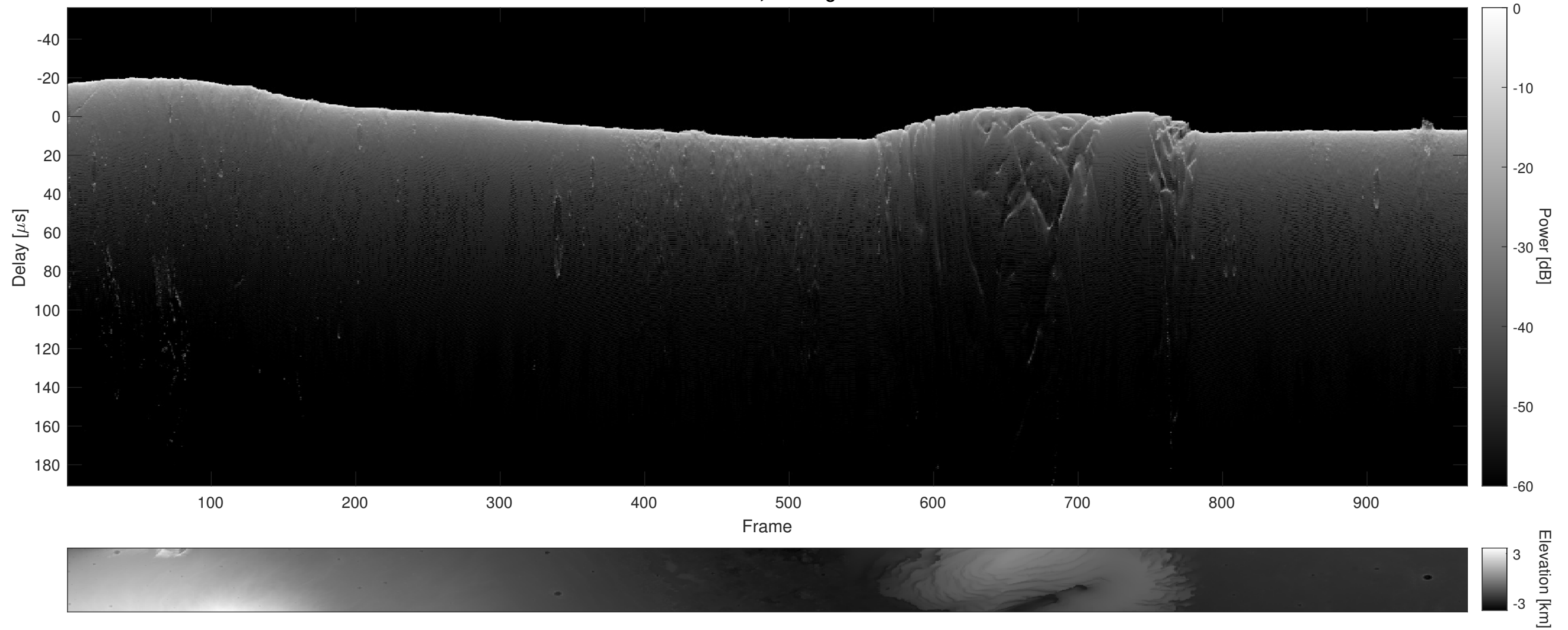
Orbit 18216, Cluttergram
