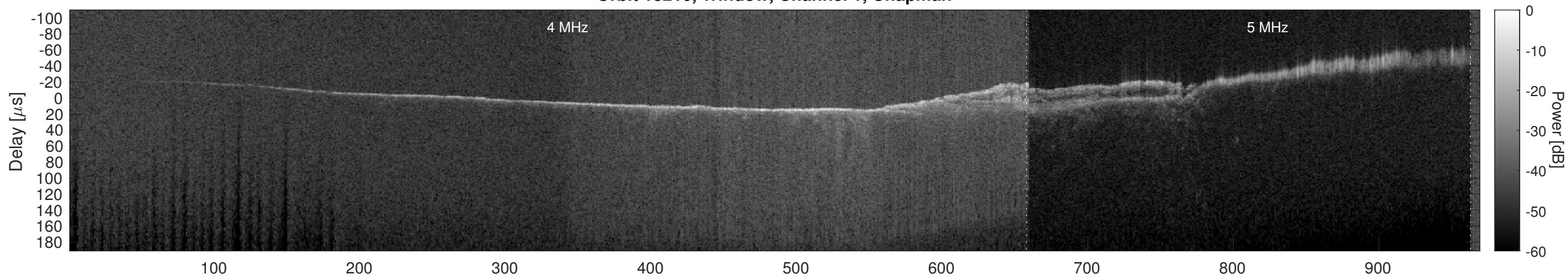
Orbit 18216, Window, Channel 1, Optimized
