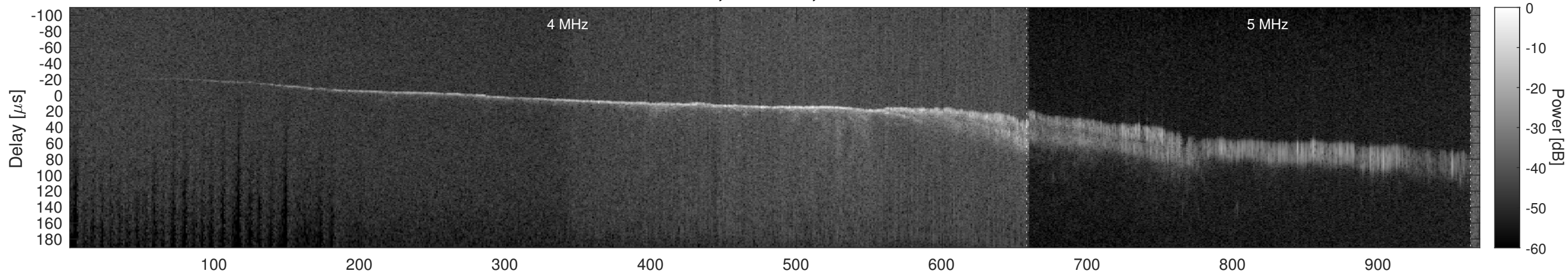
Orbit 18216, Window, Channel 1, Chapman
