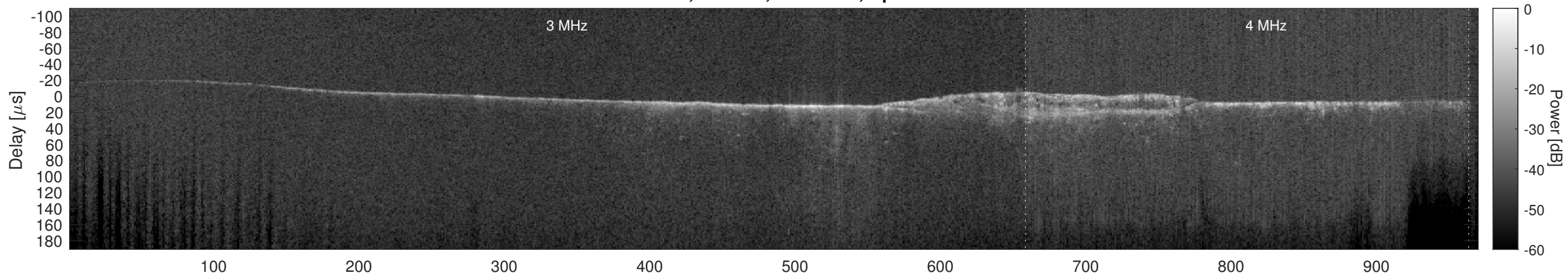
Orbit 18216, Cluttergram
