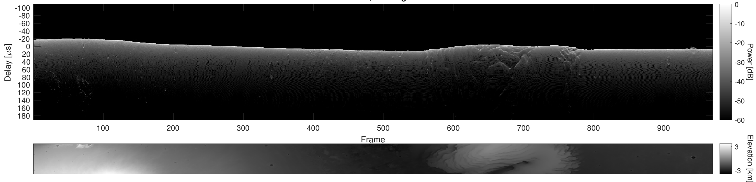
Orbit 18216, Cluttergram
