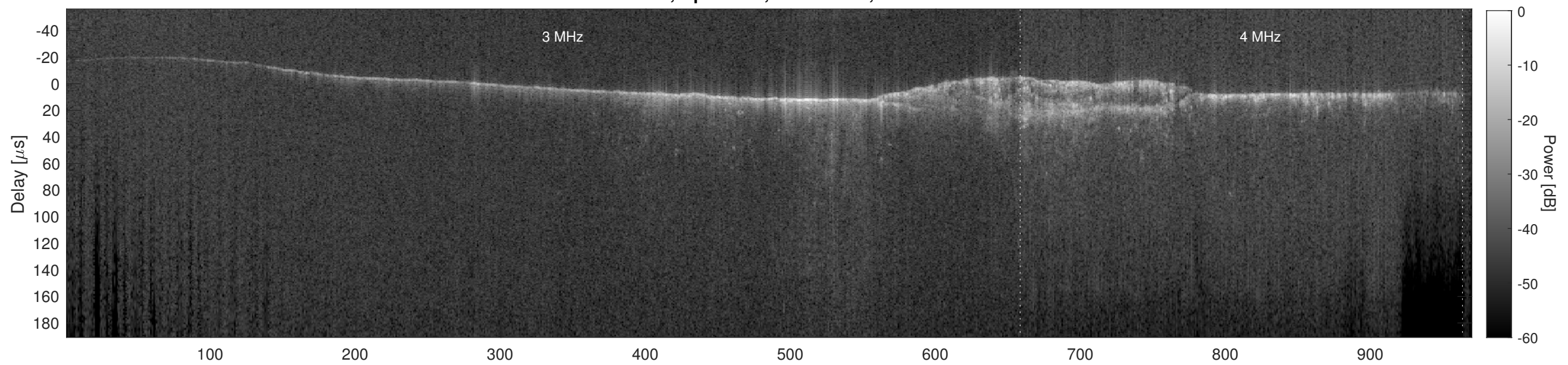
Orbit 18216, Cluttergram
