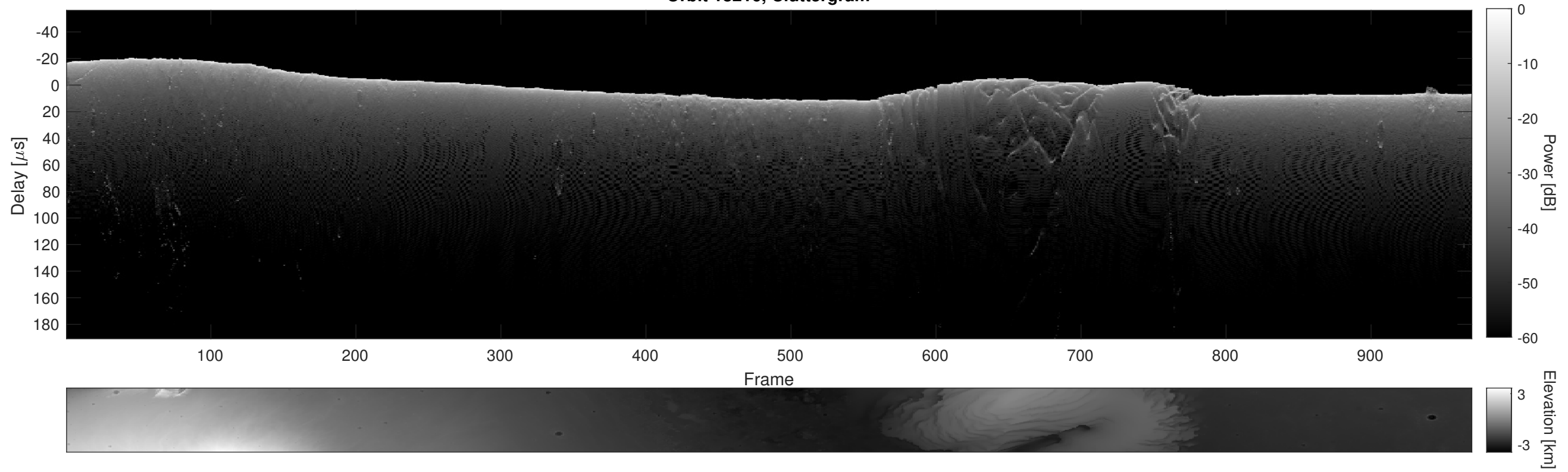
Orbit 18216, Cluttergram
