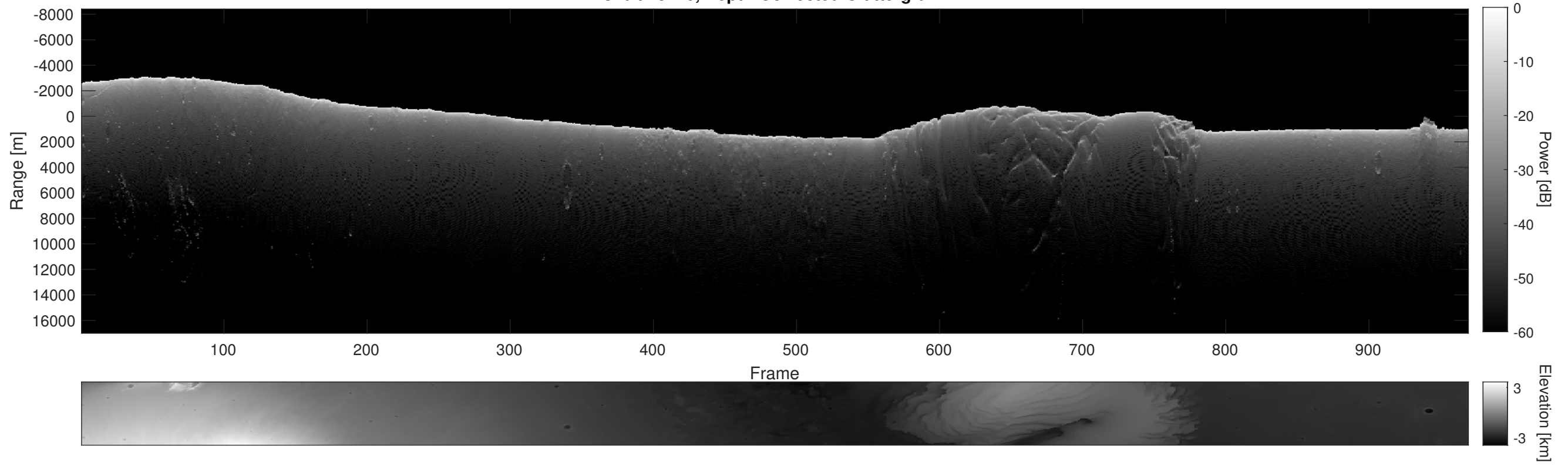
Orbit 18216, Depth-Corrected Cluttergram
