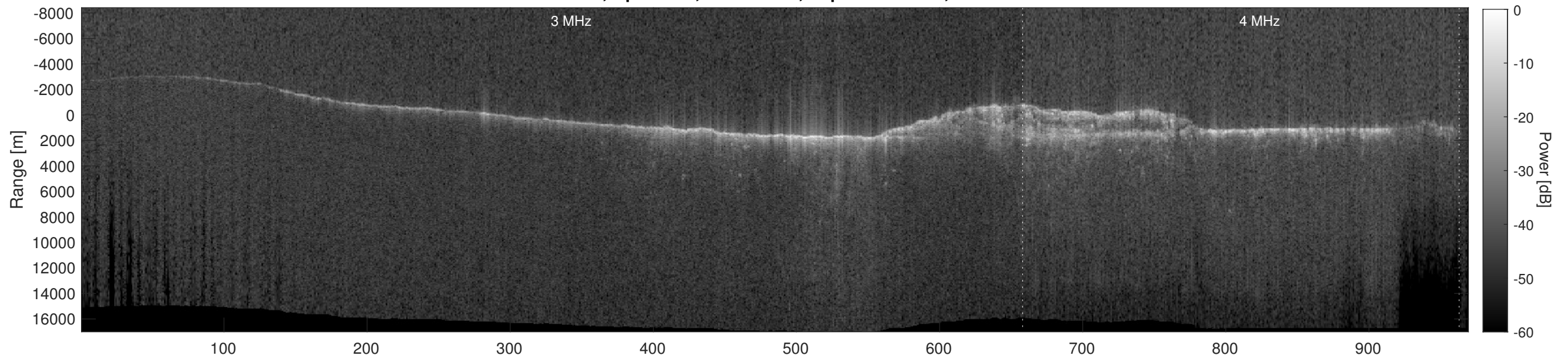
Orbit 18216, Depth-Corrected Cluttergram
