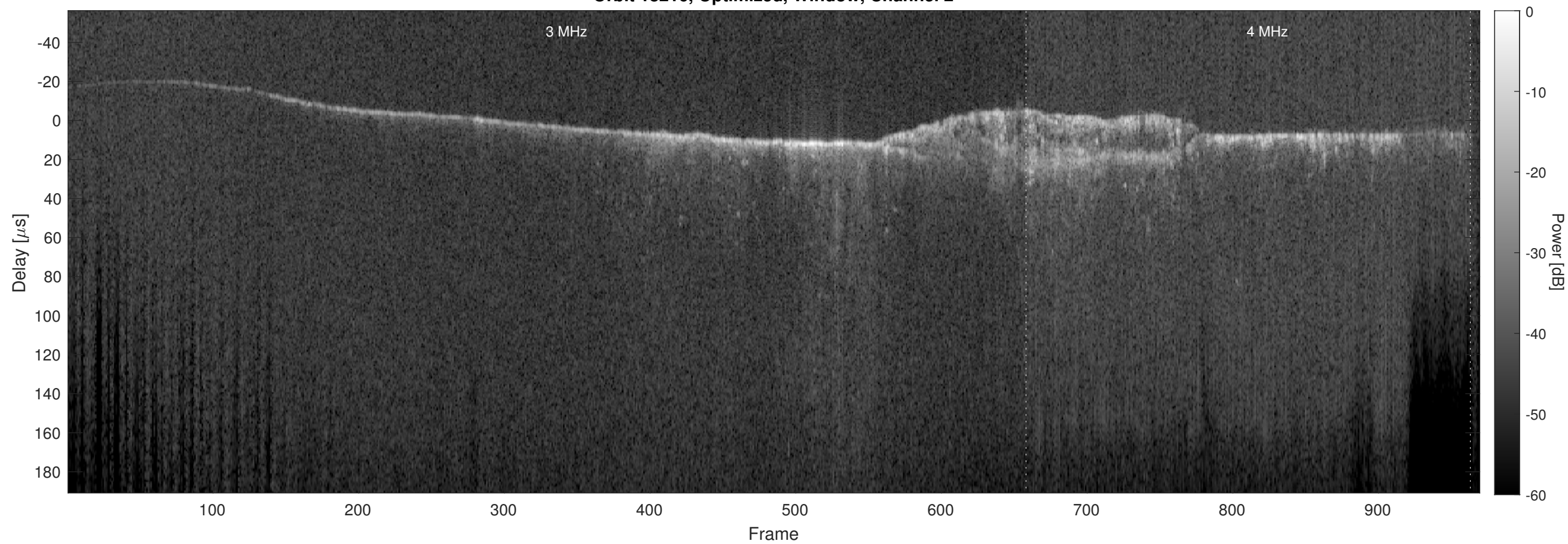
Orbit 18216, Optimized, Window, Channel 2
