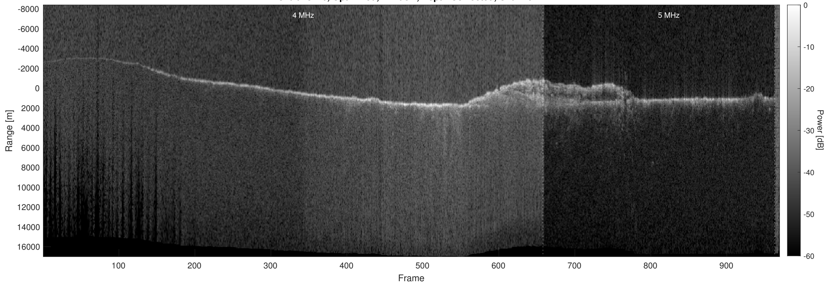
Orbit 18216, Optimized, Window, Depth-Corrected, Channel 2
