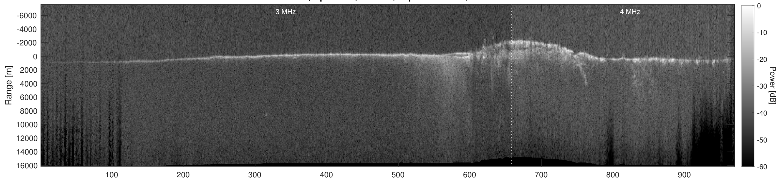
Orbit 18217, Depth-Corrected Cluttergram
