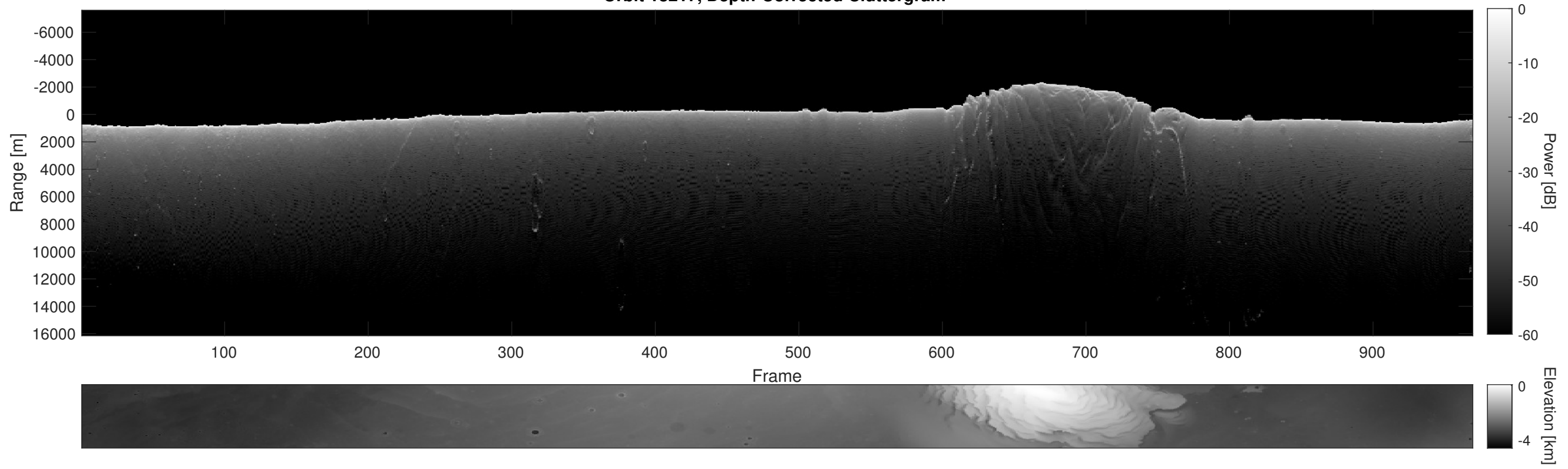
Orbit 18217, Depth-Corrected Cluttergram
