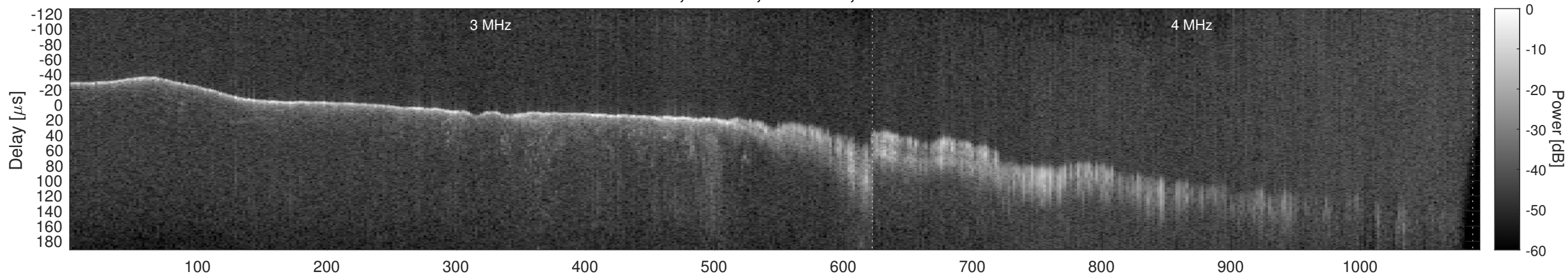
Orbit 18223, Window, Channel 2, Chapman
