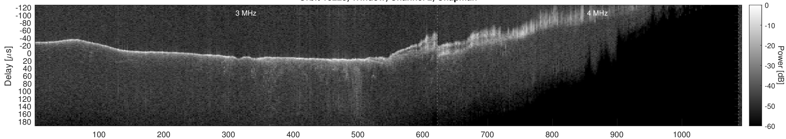
Orbit 18223, Window, Channel 2, Optimized
