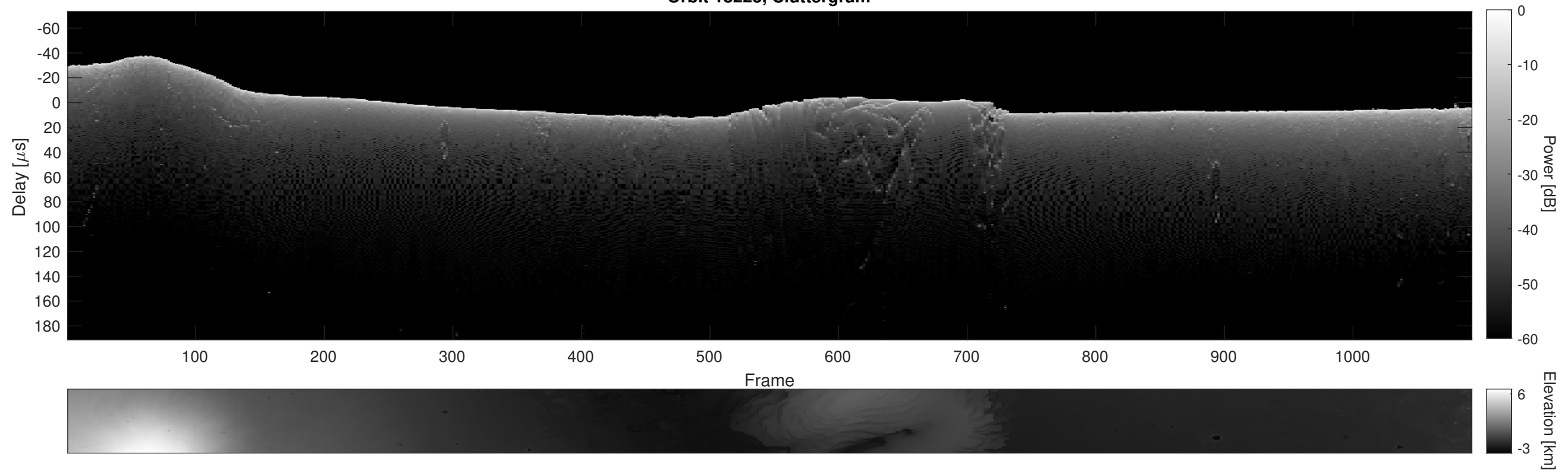
Orbit 18223, Cluttergram
