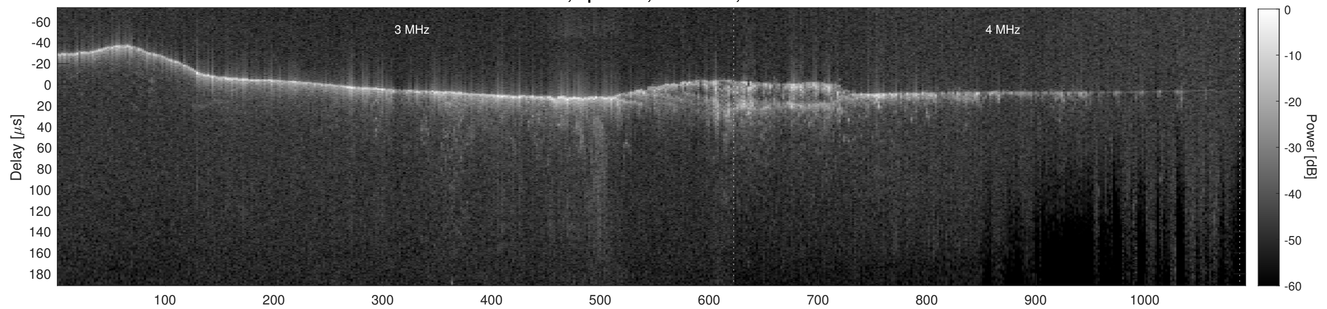
Orbit 18223, Cluttergram
