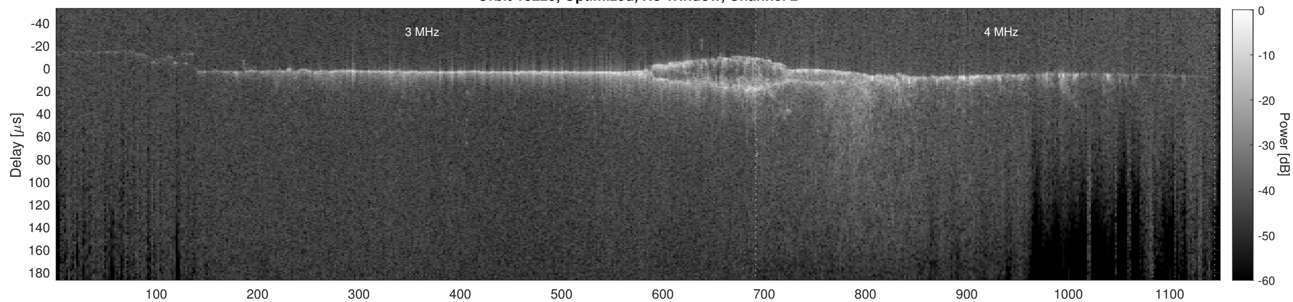
Orbit 18225, Cluttergram
