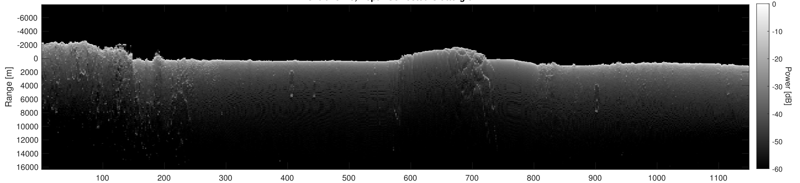
Orbit 18225, Depth-Corrected Cluttergram
