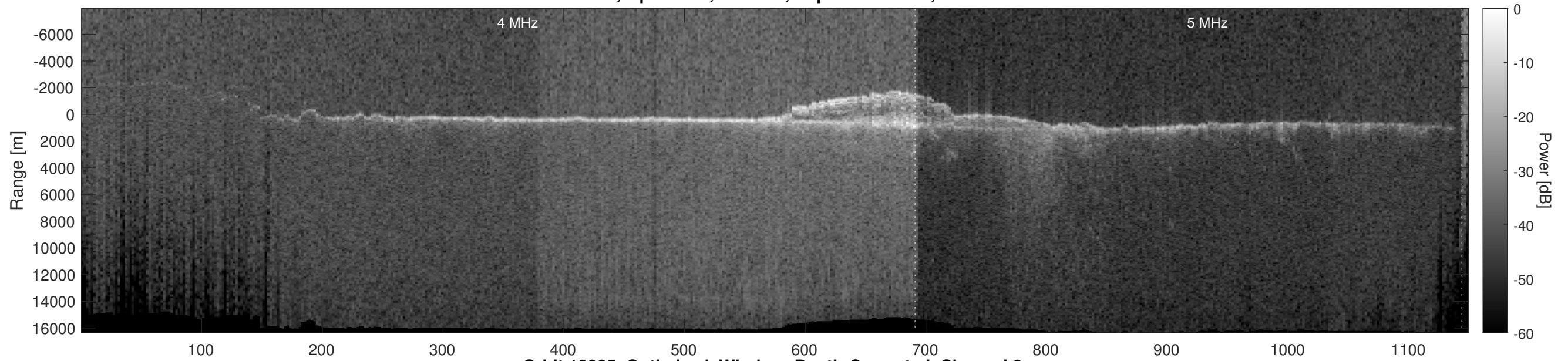
Orbit 18225, Optimized, Window, Depth-Corrected, Channel 2
