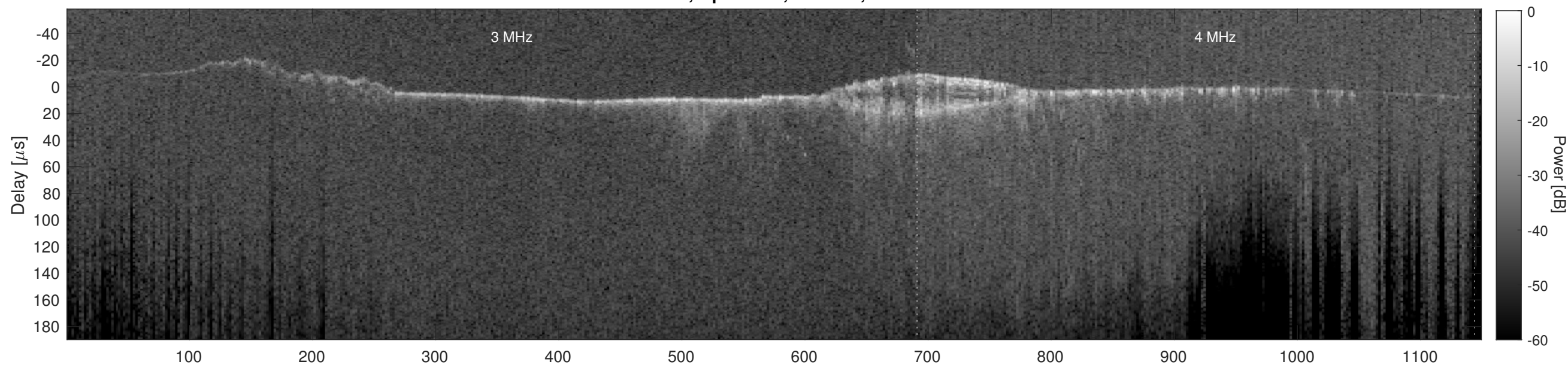
Orbit 18226, Cluttergram
