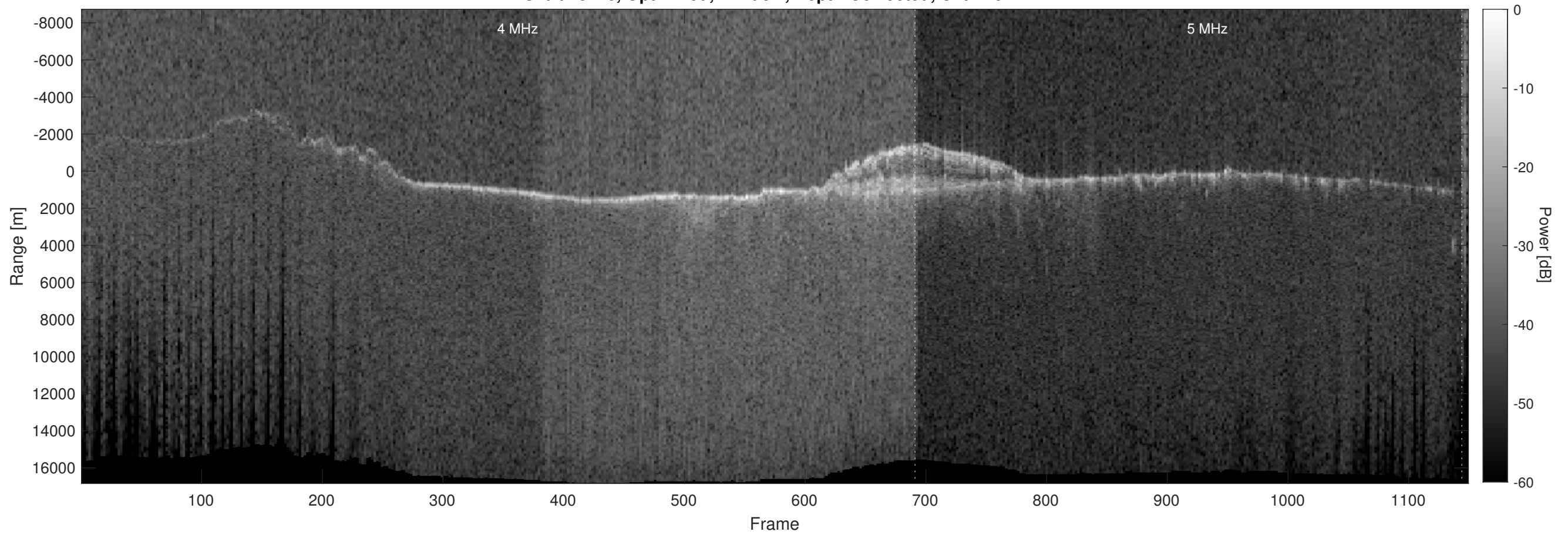
Orbit 18226, Optimized, Window, Depth-Corrected, Channel 2
