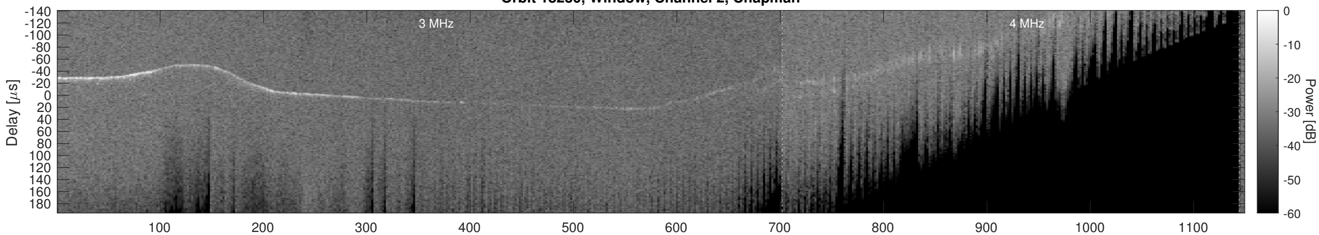
Orbit 18230, Window, Channel 2, Optimized
