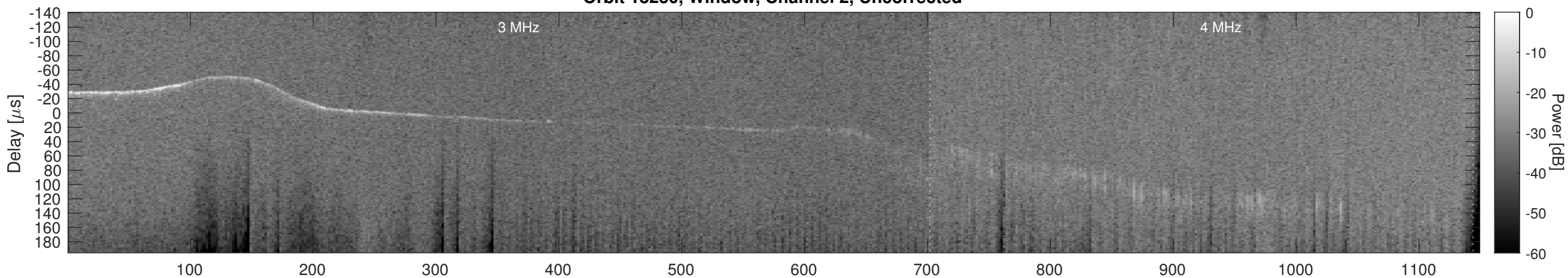
Orbit 18230, Window, Channel 2, Chapman
