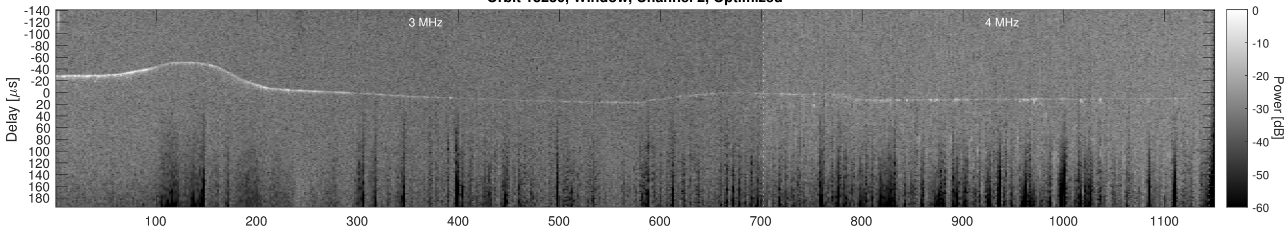
Orbit 18230, Cluttergram
