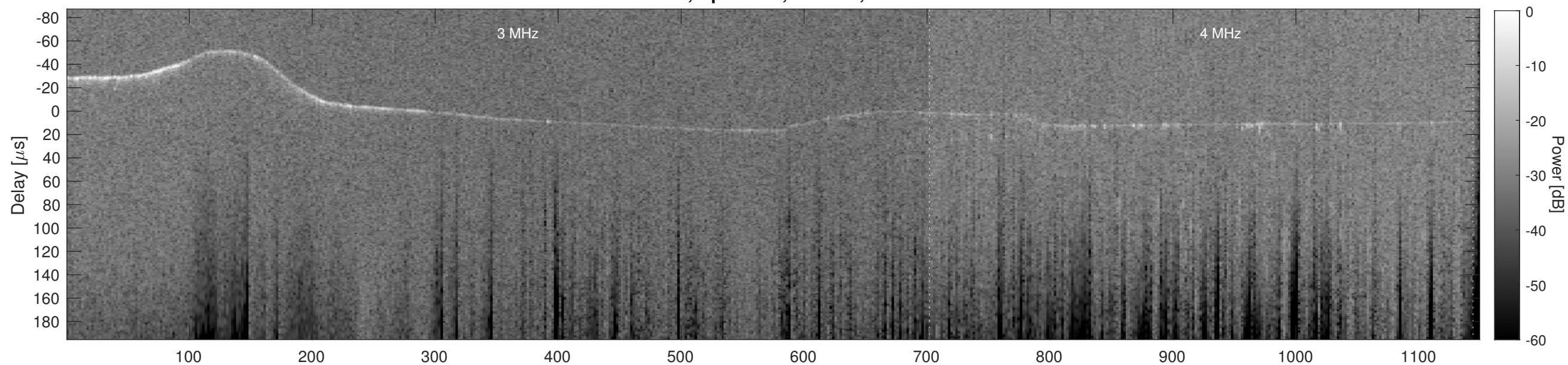
Orbit 18230, Cluttergram
