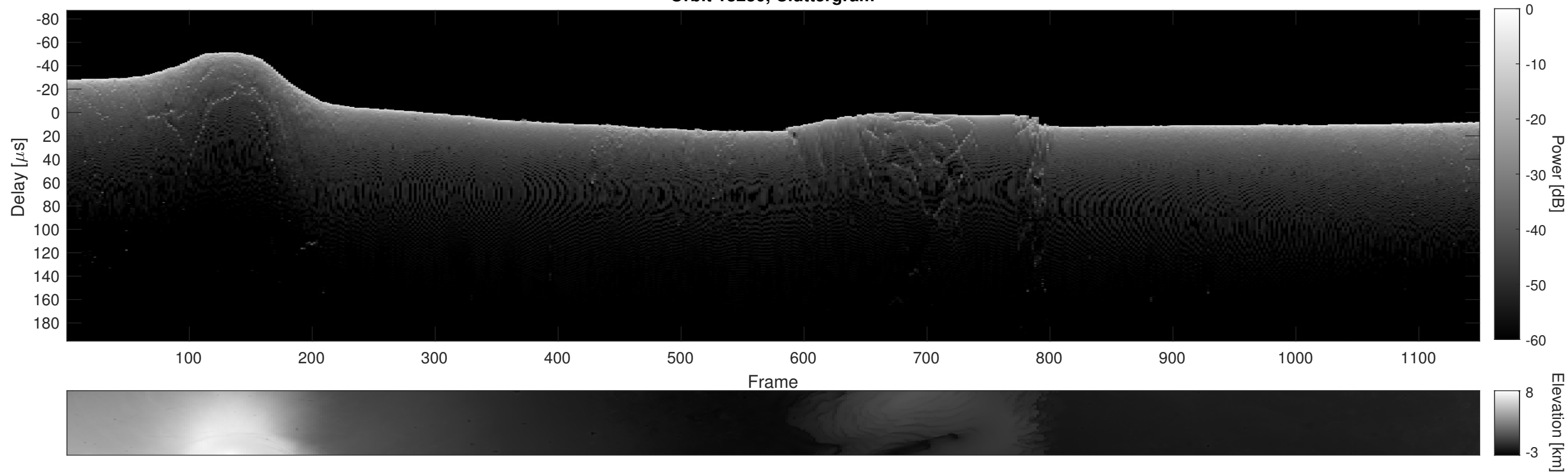
Orbit 18230, Cluttergram
